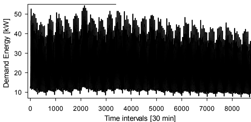
Fig. 2. Building energy demand
