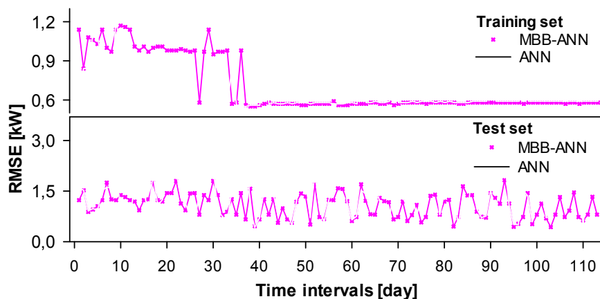
Fig. 8. Cross-validation of one-day forecast
