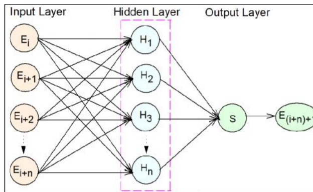
Fig. 7. Neural-network architecture
