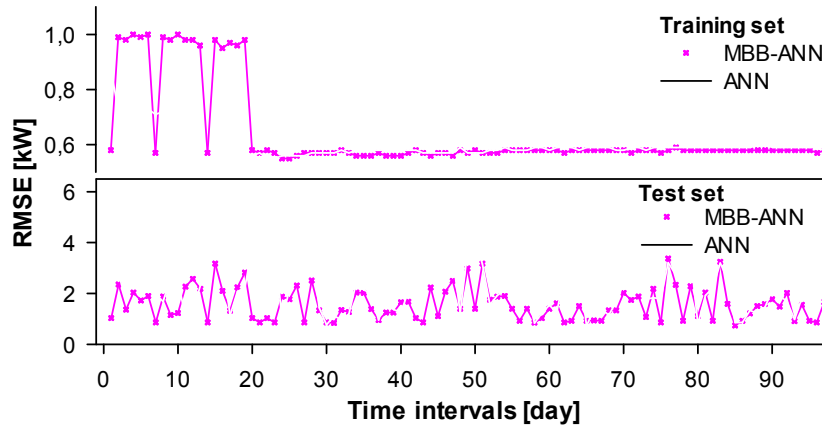
Fig. 10. Cross-validation of three-day forecast
