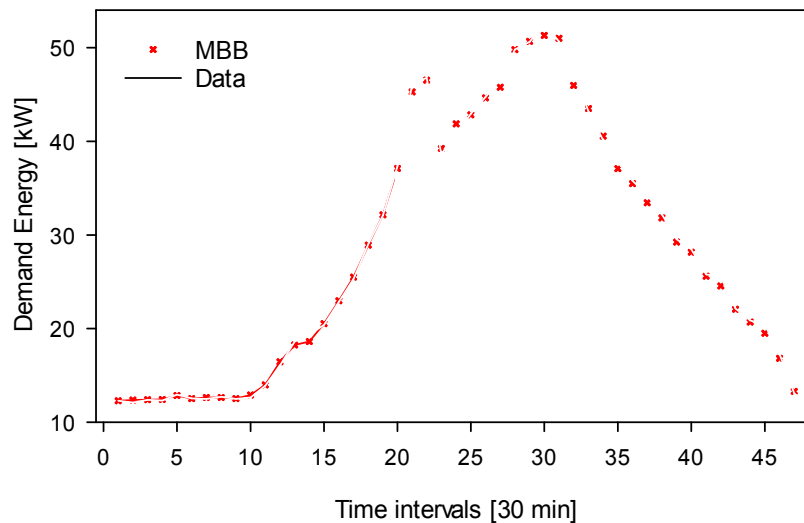
Fig. 6. Mean of bootstrapped versions for the first 48 records
