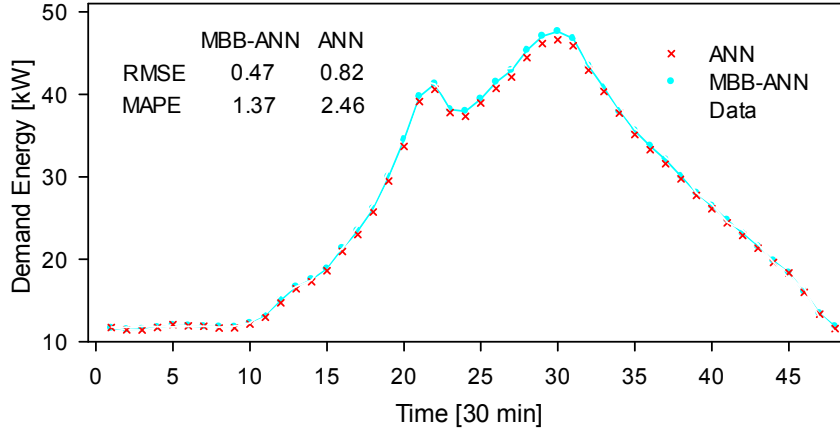
Fig. 3. Forecast one day in advance
