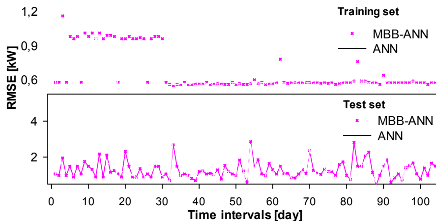
Fig. 9. Cross-validation of two-day forecast
