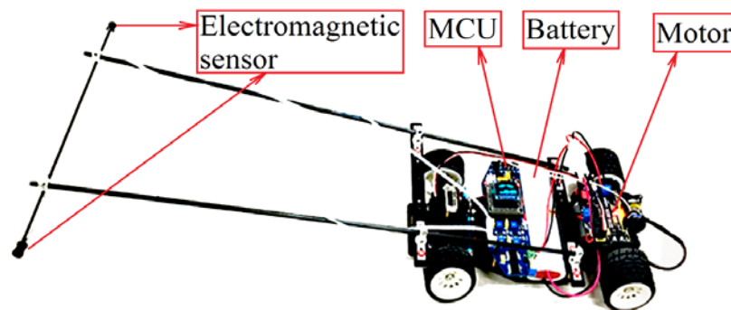
Figure 1. Electromagnetic car
