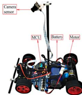
Figure 2. Camera car
