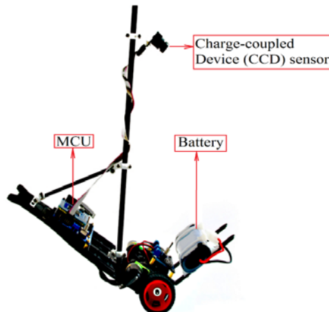
Figure 3. Photo-electric car
