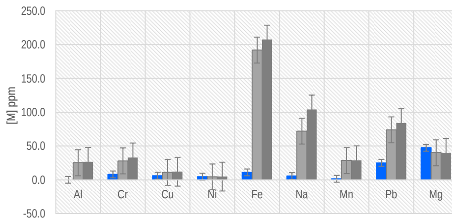
Figure 5. Variation in metal content, 1 al 11, series 1-6-7
