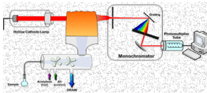
Figure 2. Atomic Absorption Spectroscopy
