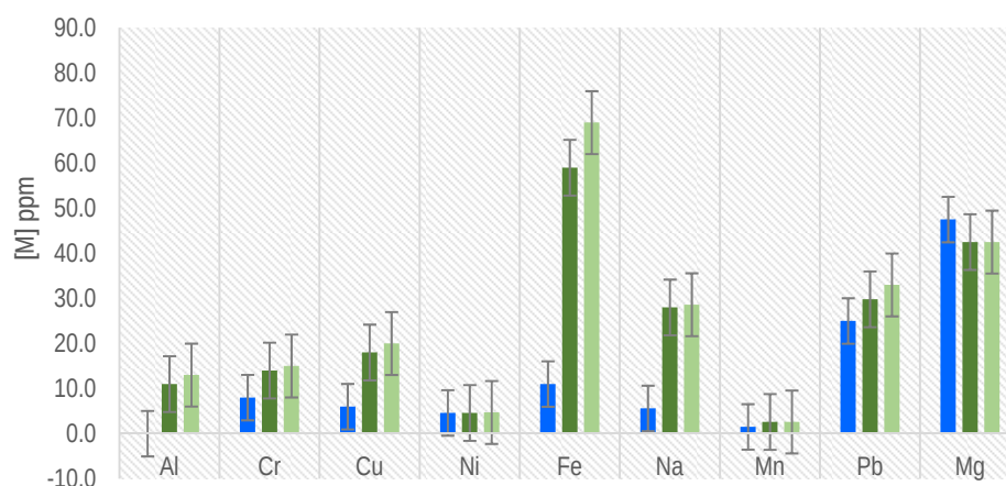
Figure 4. Variation in metal content, 1 al 11, series 1-4-5
