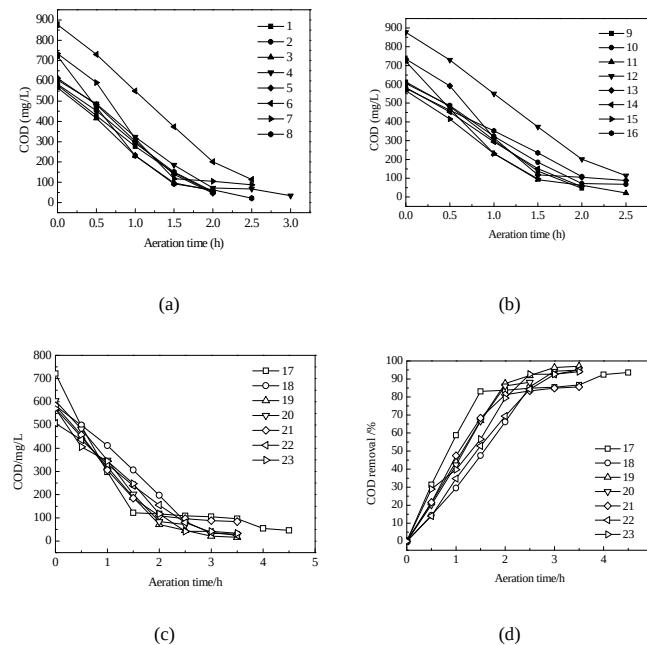
Fig.5 Effects of aeration time on COD
