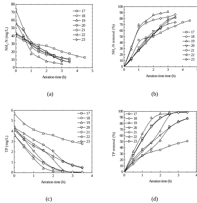
Fig.6 Effects of aeration time on NH 3 -N and total phosphorus
