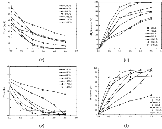
Fig.4 Effects of air flow on COD, \text{NH}_3\text{-N} and TP
