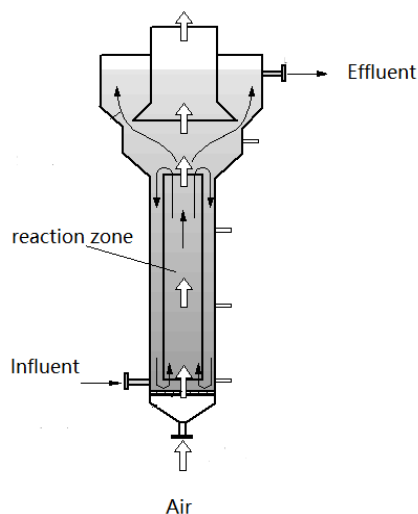
Fig.1 Schematic diagram of the apparatus
