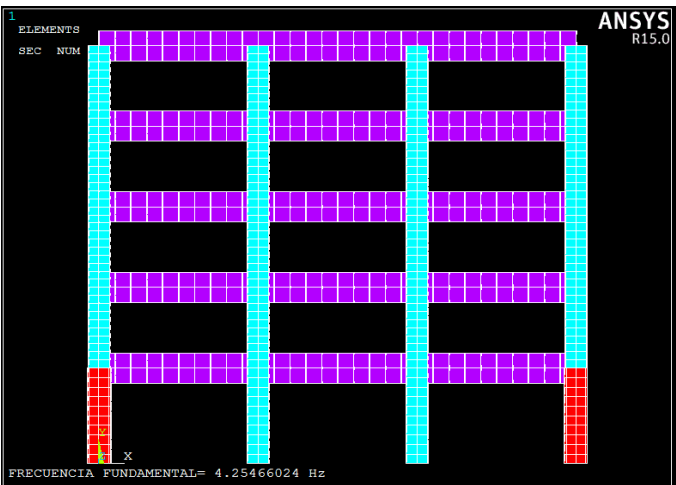
247 248 Fig. 6. Five-story building with damage in the first story
