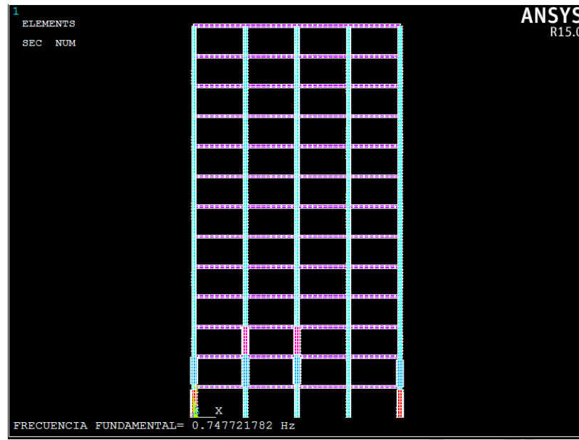
Fig. 14. 13-story building with damage on the four first stories
