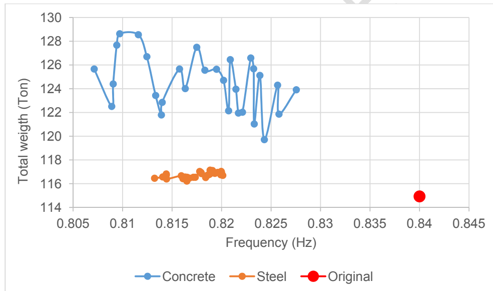
Fig. 17. Variation of the weight of the rehabilitated 13-story non-regular building with respect to its resonance frequencies. The Damage occurs on the four first stories. Case1: Reinforcement concrete jacketing, case 2: Reinforcement Steel jacketing, case 3: No additional reinforcement
