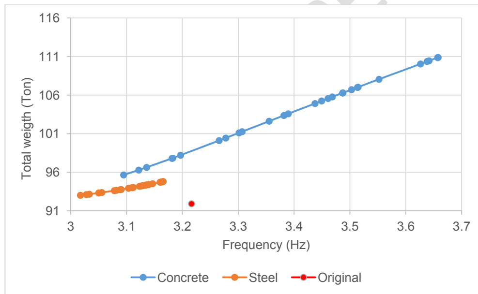
Fig. 9. Variation of the weight of the rehabilitated Two-story building with respect to its resonance frequencies. The Damage occurs on the first story. Case1: Reinforcement concrete jacketing, case 2: Reinforcement Steel jacketing, case 3: No additional reinforcement
