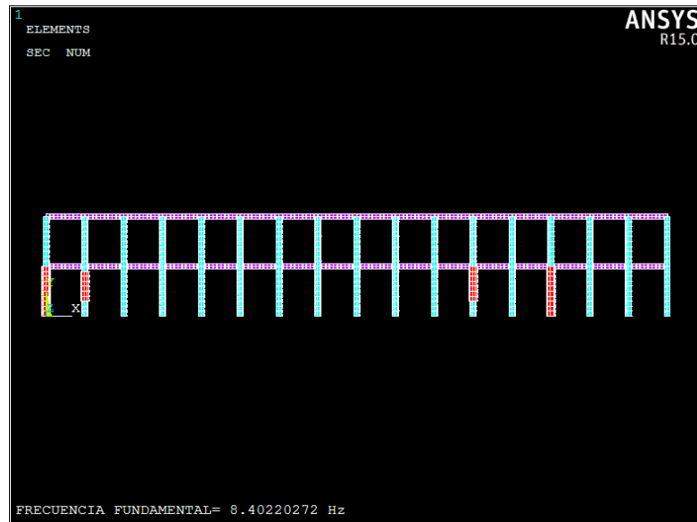
Fig. 8. Two-story building with damage in the first story
