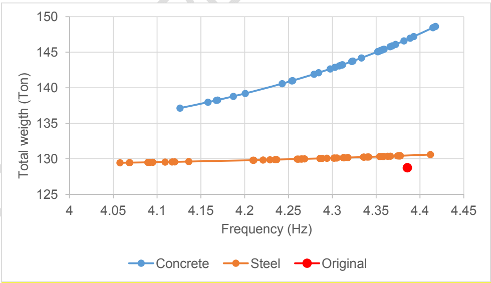
249 250 Fig. 7. Variation of the weight of the rehabilitated Five-story building with respect to its 251 resonance frequencies. The Damage occurs on the first story. Case1: Reinforcement concrete 252 jacketing, case 2: Reinforcement Steel jacketing, case 3: No additional reinforcement
