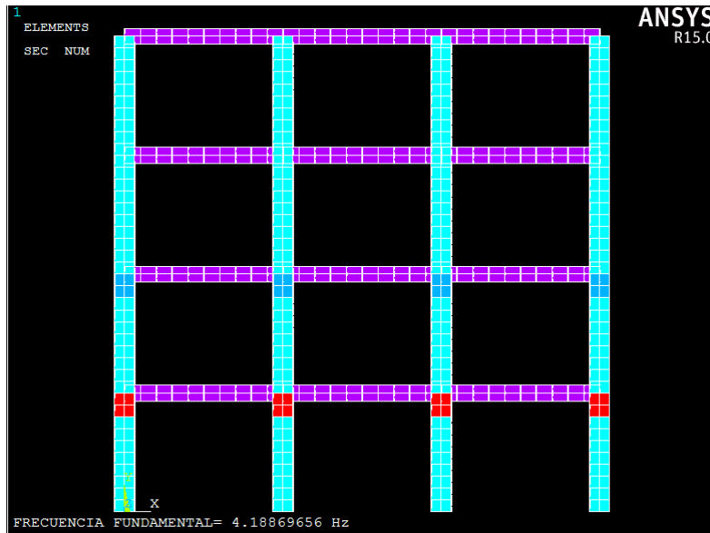
Fig. 10. Four-story building with damages in the first two stories
