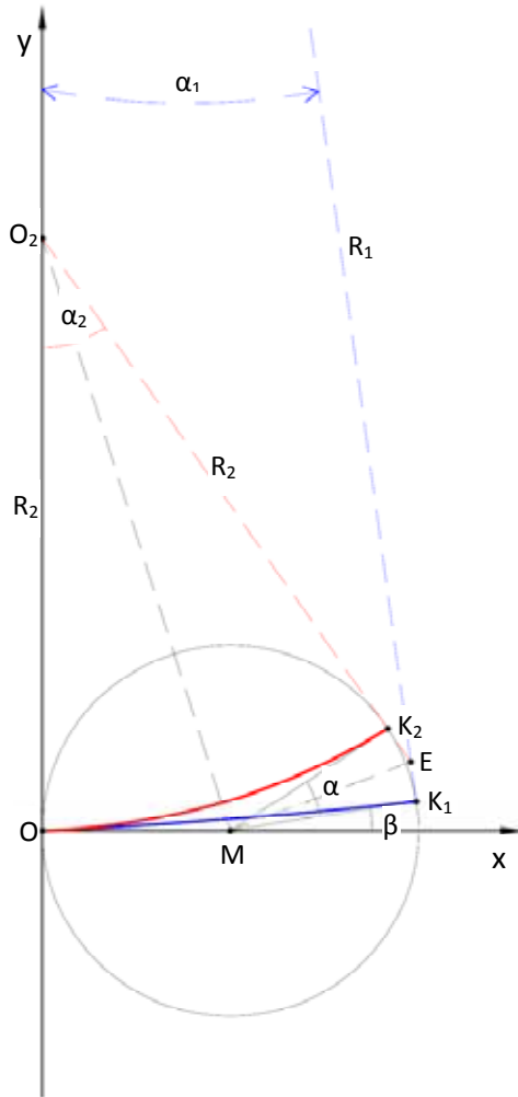
Fig. 4. A scheme of an ordinary turnout arching in variant I
