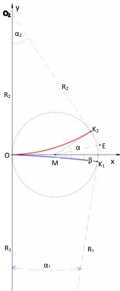
Fig. 6. A scheme of an ordinary turnout arching in variant II
