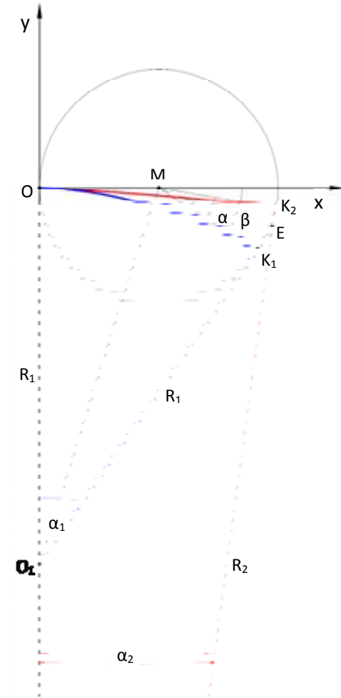
Fig. 8. A scheme of an ordinary turnout arching in variant III
