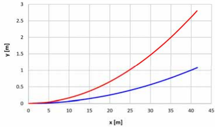
Fig. 5. Diagrams of horizontal ordinates of the main track (blue colour) and the diverging one (red colour) for variant I while arching the turnout 1 : 12 – 500 ( R_1 = 800 m, R_2 = 307.360 m, using different scales)
