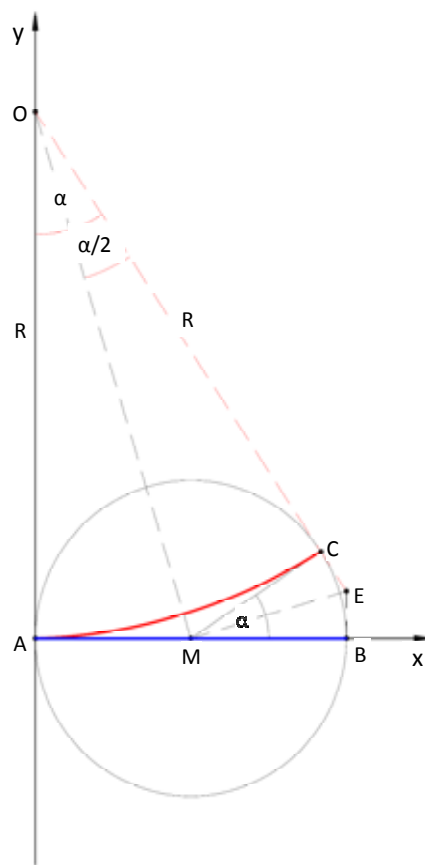
156 157 Fig. 3. Diagram of an ordinary turnout prior to its arc formation 158
