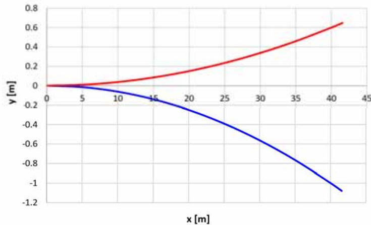
308 Fig. 7. Diagrams of horizontal ordinates of the main track (blue colour) and the 309 diverging one (red colour) for variant II while arching the turnout 1 : 12 – 500
