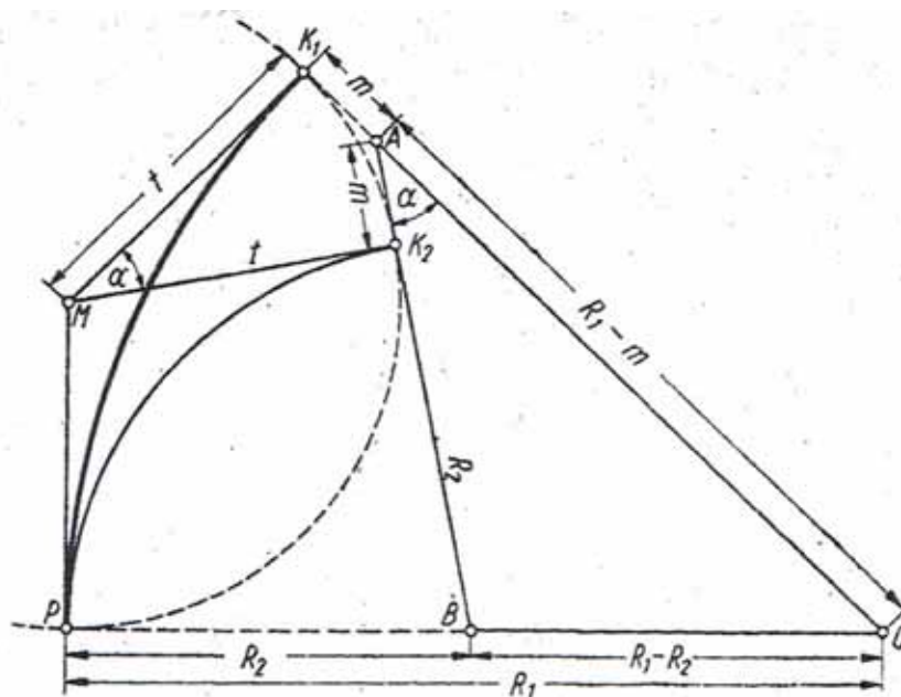
97 Fig. 2. A scheme for the determination of the diverging track radius in the one-sided 98 curved turnout (according to paper [12])
