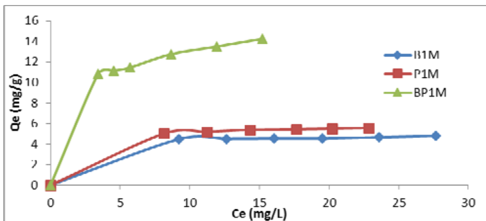
Fig.11. Effect of initial concentration on adsorbed quantities
