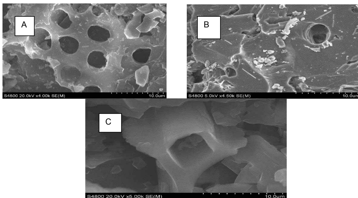
Fig. 1. The SEM photograph of the prepared activated carbons (A: B1M, B: P1M and C: BP1M).
