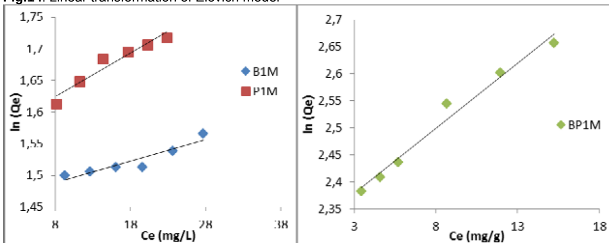
Fig. 15. Linear transformation of the Jovanovic model
