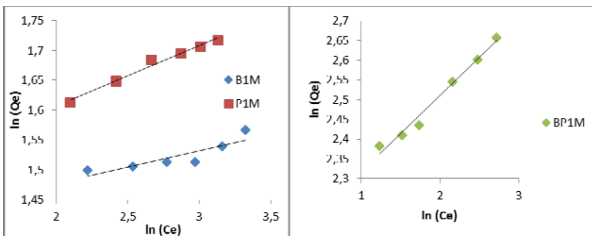
Fig.13. Linear transformation of Freundlich model
