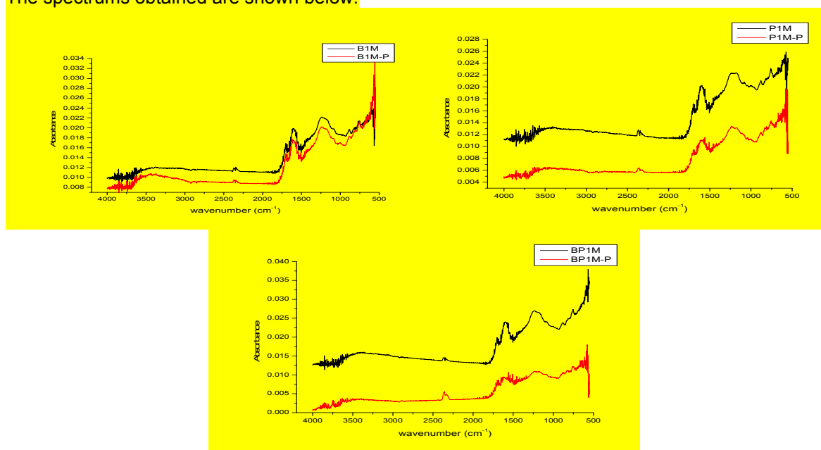
Fig 3: FT-IR Spectra of activated carbon without adsorption (back) and after adsorption (Red).
