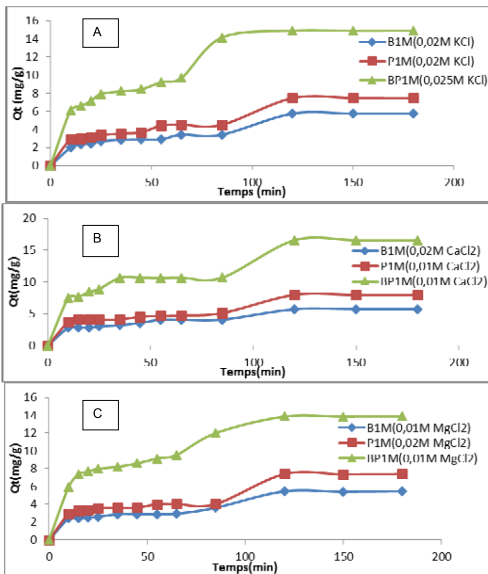
316 Fig. 7. Effect of salts on the contact time (A: effect of KCl, B: effect of \text{CaCl}_2 and C: effect of \text{MgCl}_2 ) 317
