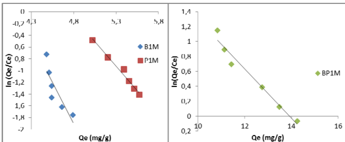
Fig.14. Linear transformation of Elovich model
