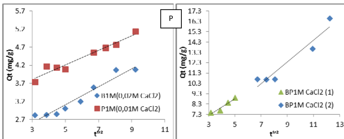
Fig. 9: Weber & Morris intraparticle diffusion (M: no sel, N: with KCl, O: with CaCl 2 , P: with MgCl 2 ) plots.
