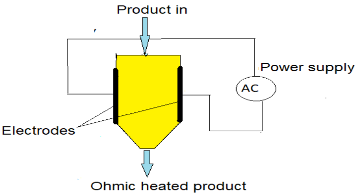
Fig. 1 - The principle of ohmic heating
