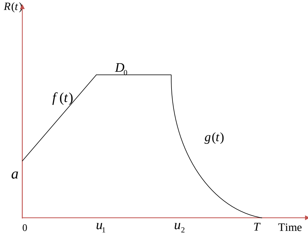
Fig. 1 Trapezoidal Demand
