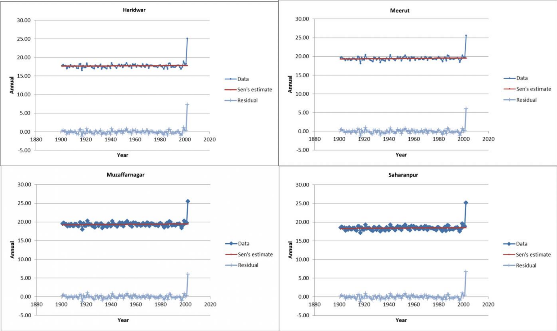
Fig 3c: Average Temperature Trend in Upper Ganga Canal Command region is presented station wise (1901-2002)
