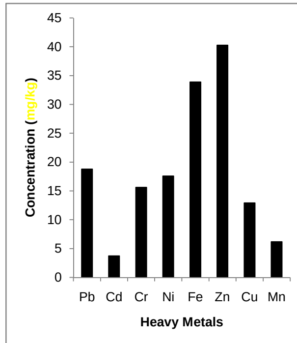
Fig. 2: Mean concentrations of the Heavy metals (mg/kg) at the mining sites Values represent Mean \pm Standard deviation of twelve determinations
