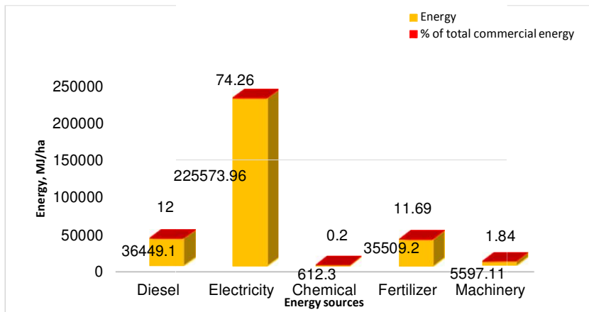
Fig 3.3 Commercial energy sources (MJ/ha) in Narsinghpur from 2013 to 2016
