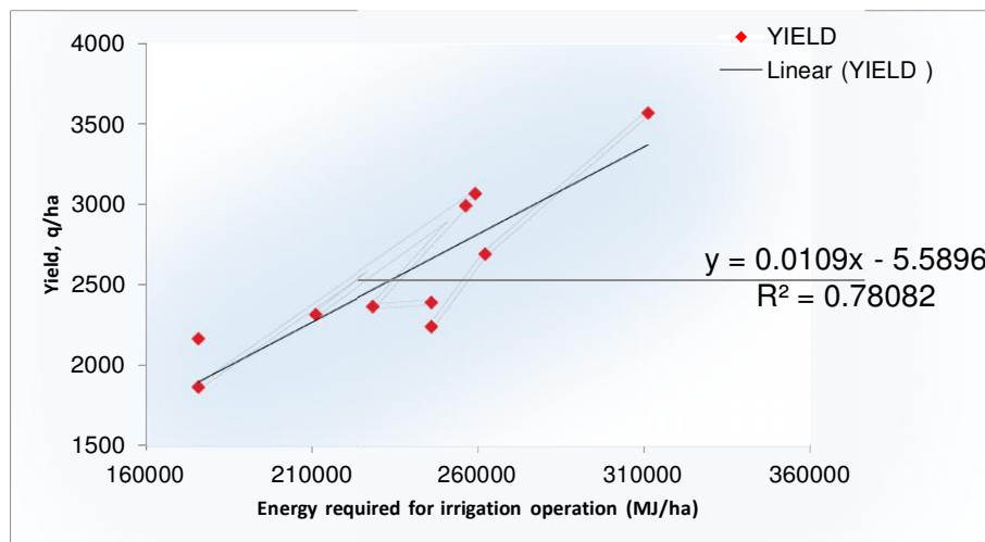
314 Fig. 3.5 Effect of irrigation on the yield of sugarcane (Narsinghpur, 2013-16)
