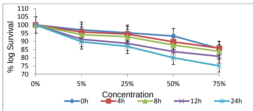
Figure 2: show the Percentage Logarithm Survival of Pseudomonas sp. with Nokia phone battery in fresh water
