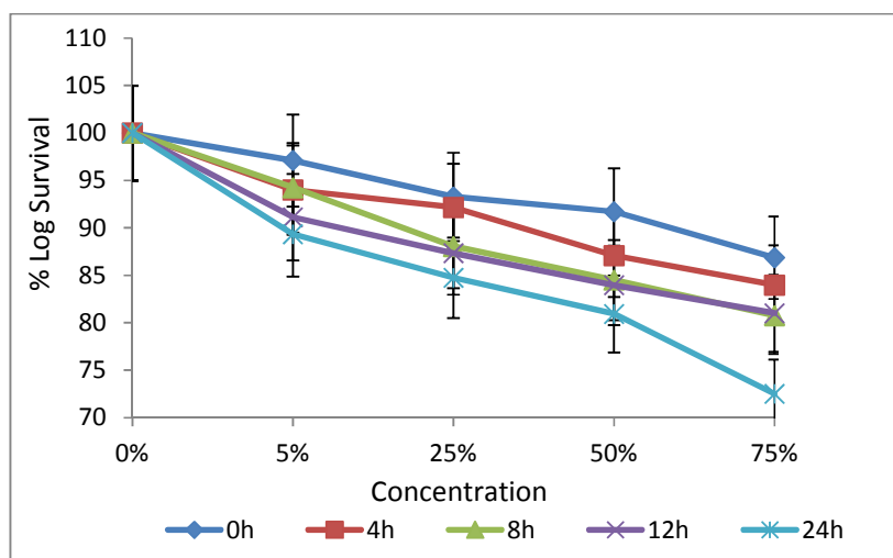
Figure 5: Lethal Toxicity of Tecno phone battery on Pseudomonas sp. in Fresh water
