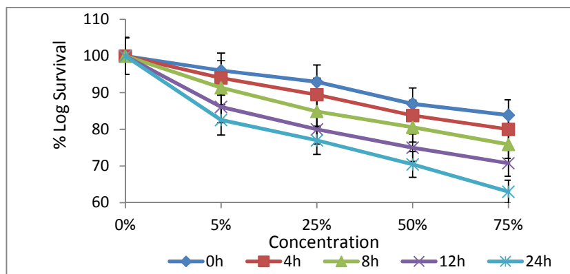
Figure 7: Lethal Toxicity of Tecno phone battery on Pseudomonas sp. in Marine
