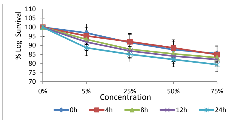
Figure 3: show the Percentage Logarithm Survival of Pseudomonas sp. with Nokia phone battery in Brackish
