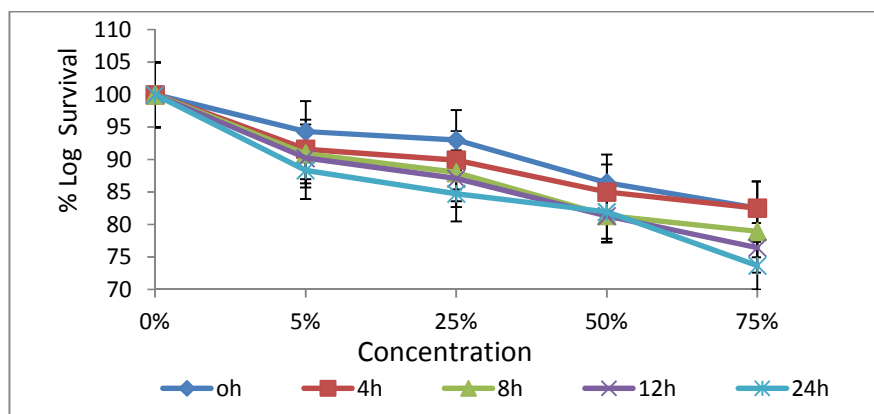
Figure 4: show the Percentage Logarithm Survival of Pseudomonas sp. with Nokia phone battery in Marine
