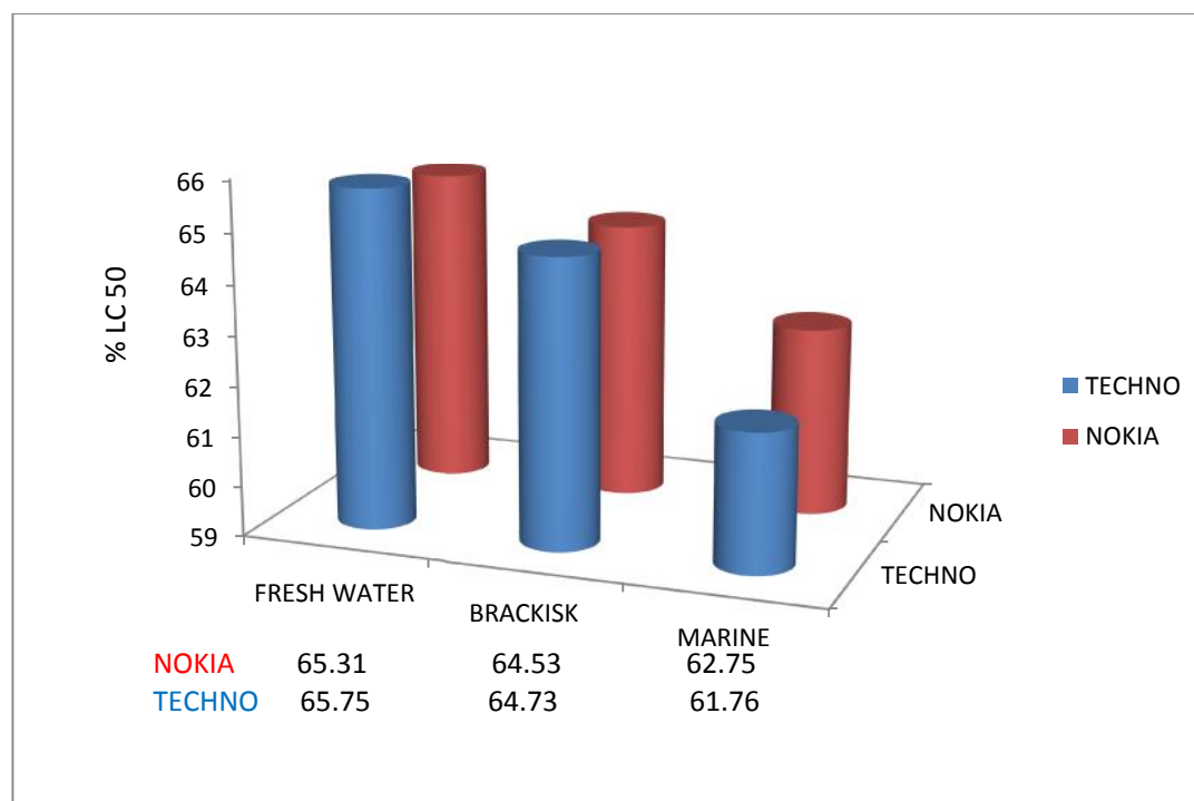
FIGURE 1: Summary of median lethal concentration of mobile phone batteries (Nokia and Techno) on Pseudomonas sp. in freshwater, brackish and marine.
