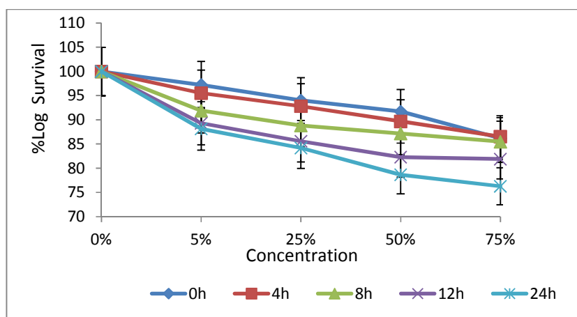
Figure 6: Lethal Toxicity of Tecno phone battery on Pseudomonas sp. in brackish
