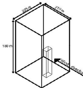
Fig. 3. Virtual wind tunnel of the CAARC model.
