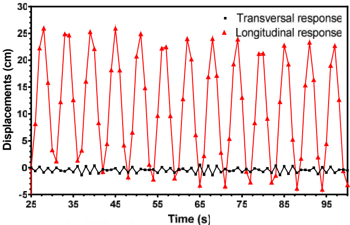
Fig. 8. Displacements in CAARC model due to dynamic wind pressures.
