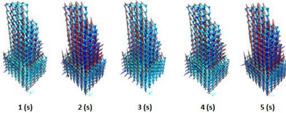
Fig. 12. Bending moment in “z” axis in time on the whole atypical geometry building model.
