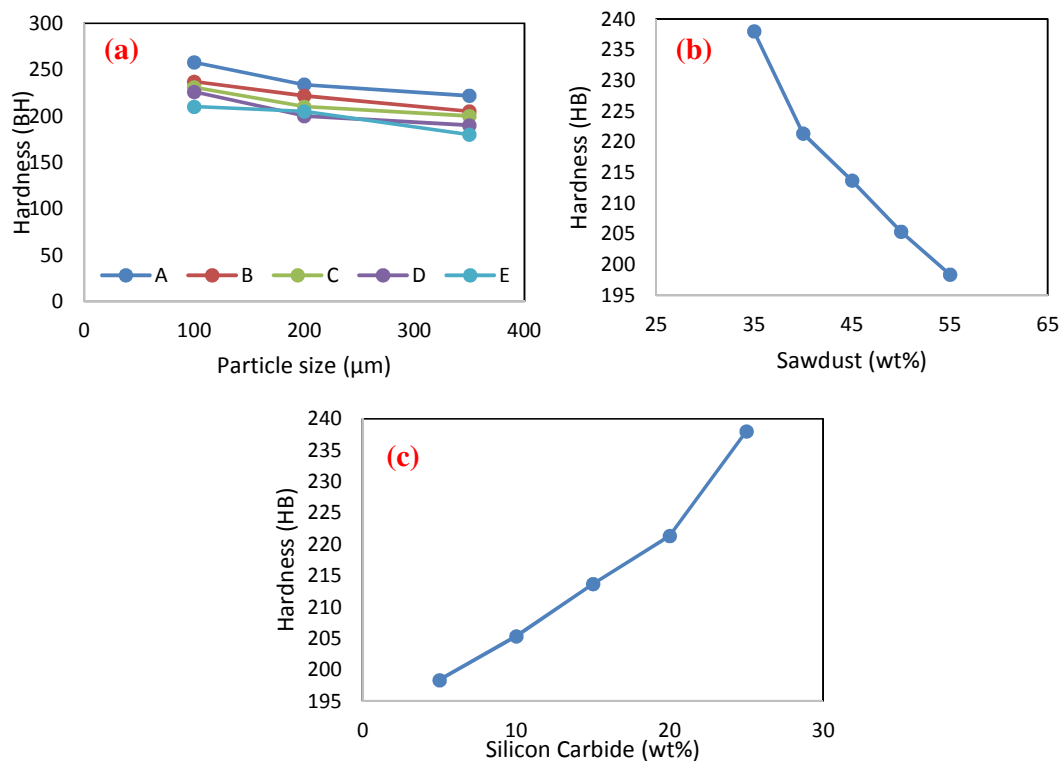
Fig.4. Hardness results as a function of (a) particle size, (b) wt% of sawdust, (c) wt% of silicon carbide
