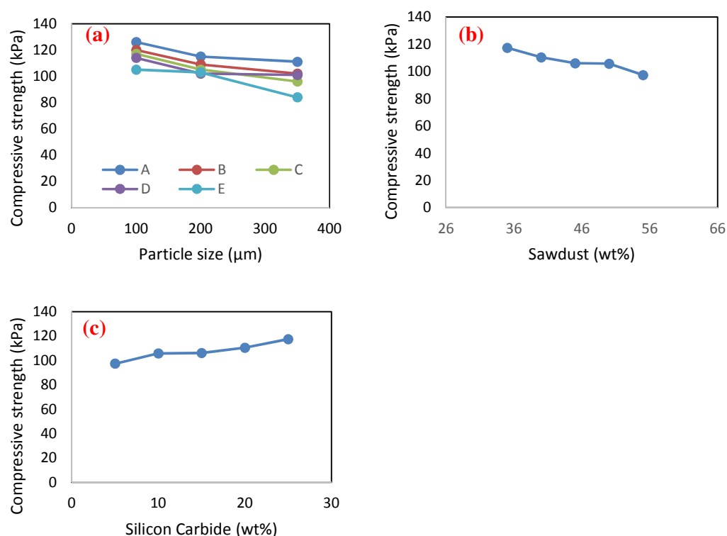
Fig.7. Correlation of compressive strength with (a) particle size, (b) wt% of sawdust, (c) wt% of silicon carbide
