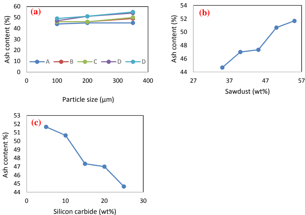
Fig.8. Relationship between ash content and (a) particle size, (b) wt% of sawdust, (c) wt% of silicon carbide
