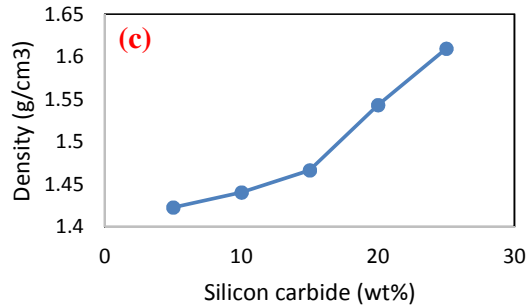
Fig.10. Relationship between density of brake pad and (a) particle size, (b) wt% of sawdust, (c) wt% of silicon carbide
