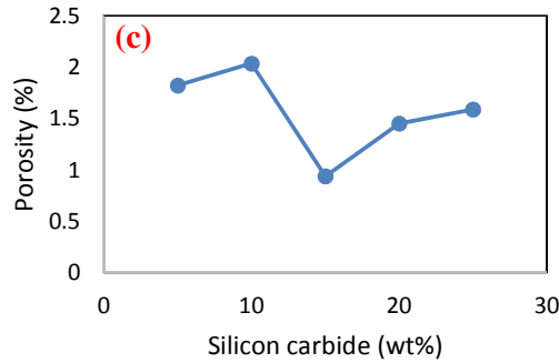
Fig.9. Relationship between porosity of brake pad and (a) particle size, (b) wt% of sawdust, (c) wt% of silicon carbide
