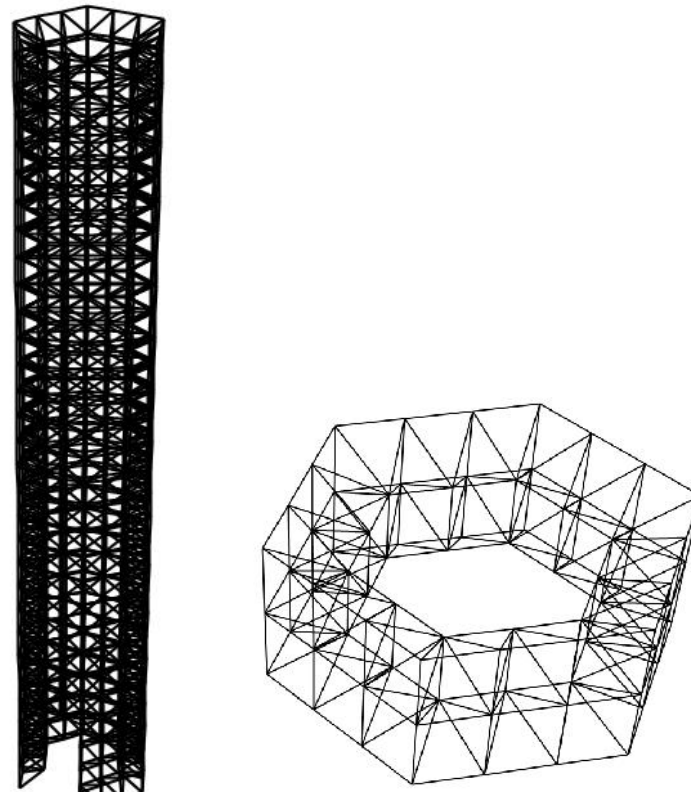
Fig. 6 Structural shape of double spatial mesh
