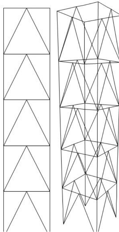
Fig. 5 Structural shape of experimental tower in Sonora.
