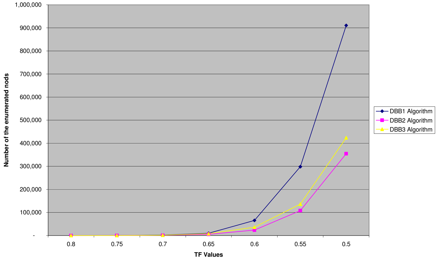
Figure 3. Effect of CTF on the number of nodes for n=15, K=4, m=3 problems
