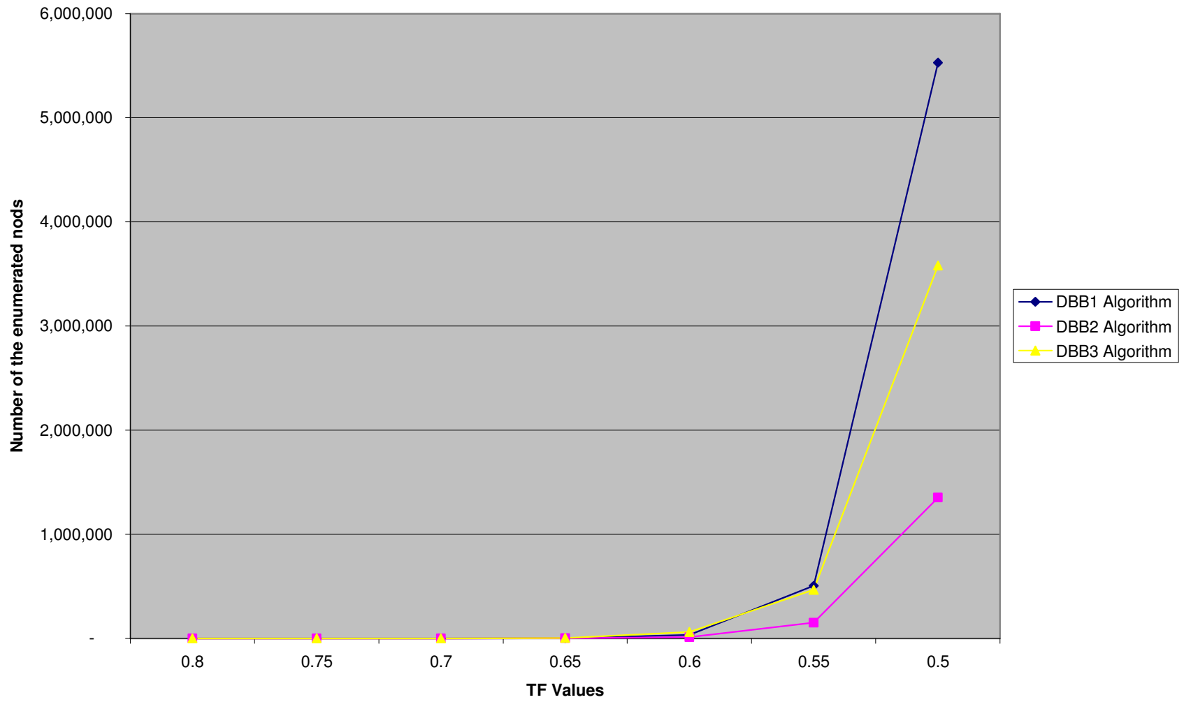
Figure 4. Effect of CTF on the number of nodes for n=20 , K=4 , m=3 problems
