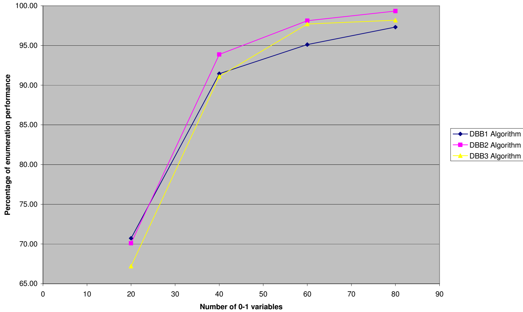
Figure 5. Performance of the developed algorithms comparing with the traditional B&B
