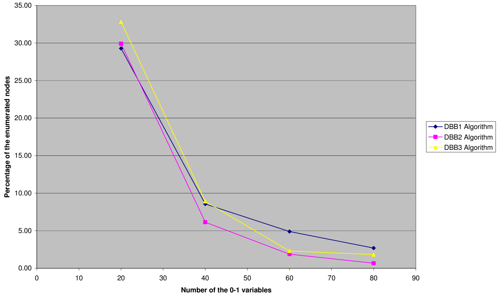
Figure 6. Percentage of the nodes enumerated by the developed algorithms comparing with the traditional B&B
