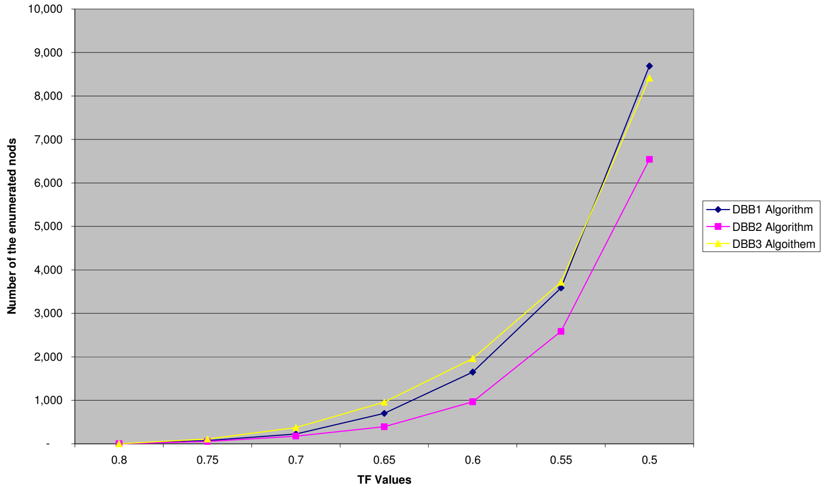
Figure 2. Effect of CTF on the number of nodes for n=10, K=4, m=3 problems
