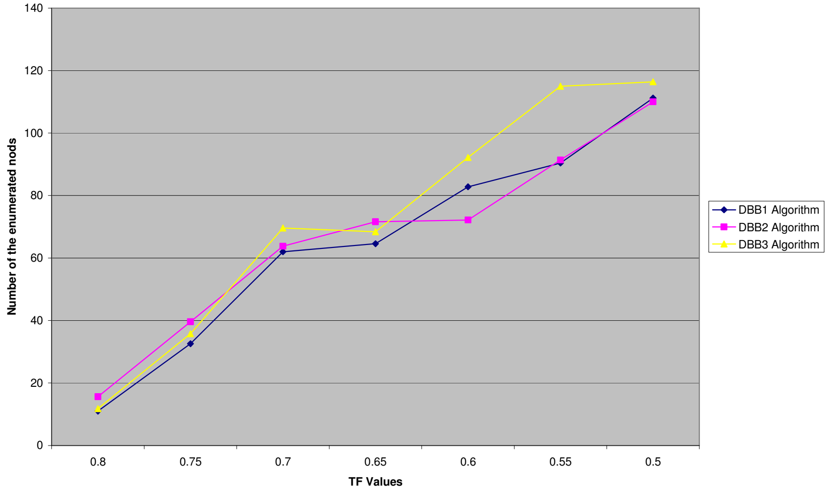
Figure 1. Effect of CTF on the number of nodes for n=5, K=4, m=3 problems
