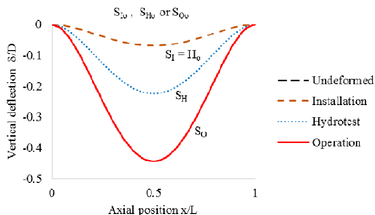
Fig. 2. Example of design sequence for fixed-fixed condition
