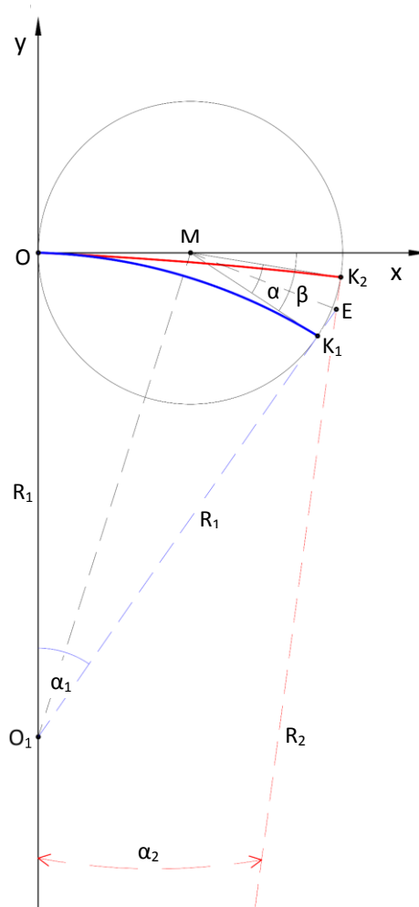
Fig. 8. A scheme of an ordinary turnout arching in variant III
