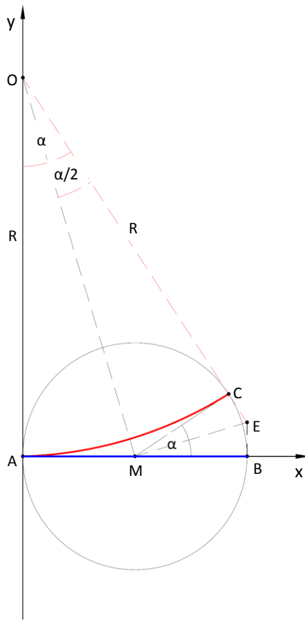
Fig. 3. Diagram of an ordinary turnout prior to its arc formation
