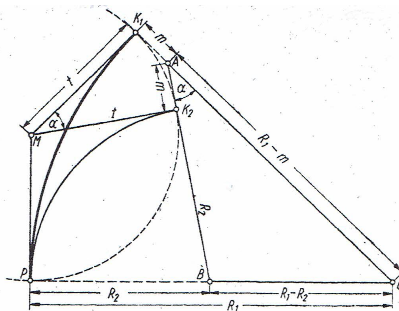
Fig. 2. A scheme for the determination of the diverging track radius in the one-sided curved turnout (according to paper [1])
