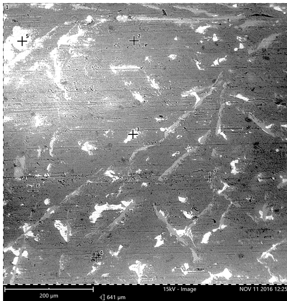
Figure 5: BSE-SEM image of the Al-4043/10 wt.% SiC composite
