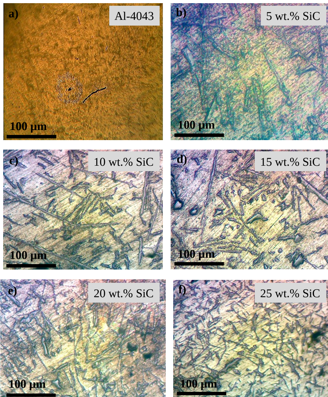
Figure 4: Optical micrographs of the Al-4043/SiC composites with varying wt.% reinforcement
