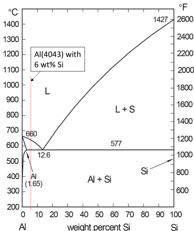
Figure 6: Al-4043 alloy located on the binary Al-Si phase diagram
