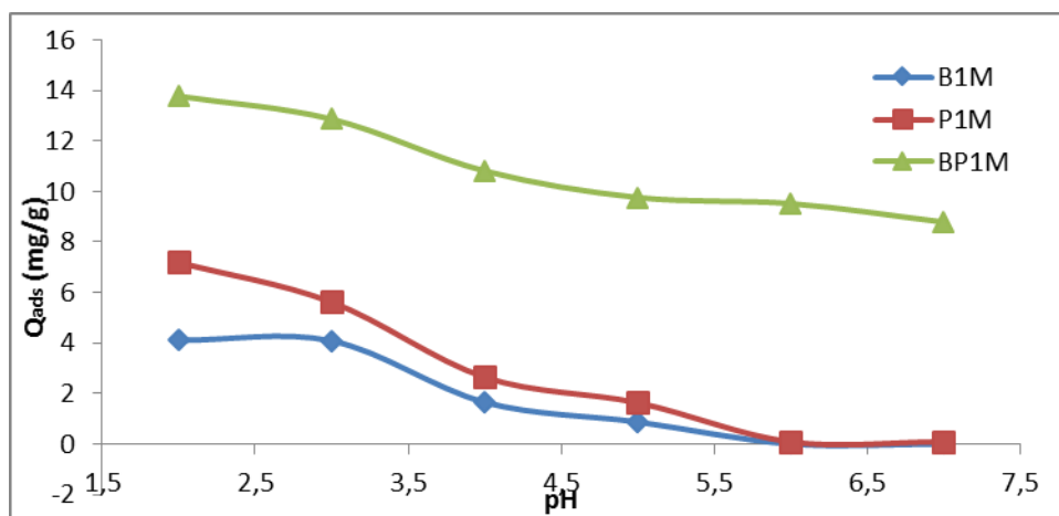
221 Fig.3. Influence of pH on the adsorption of phenacetin.
