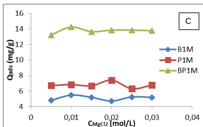
Fig. 5. Effect of initial concentration of salt on the adsorbed quantities (A: effect of KCl, B: effect of CaCl_2 and C: effect of MgCl_2 ).
