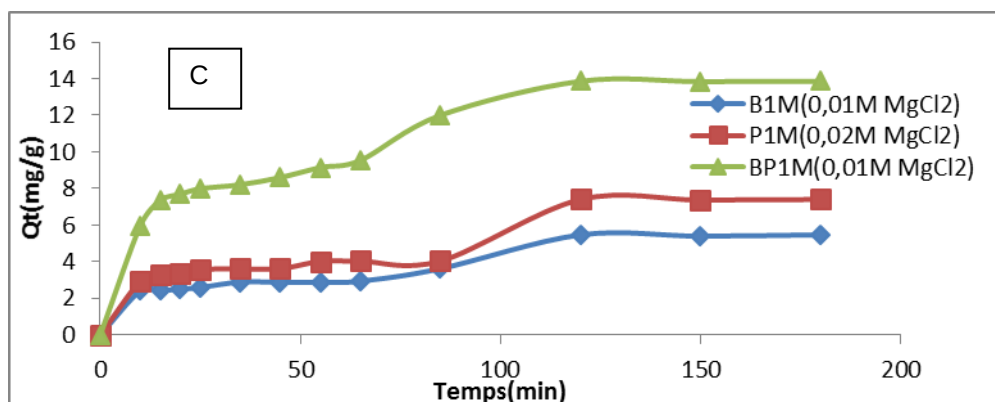
Fig. 6. Effect of salts on the contact time (A: effect of KCl, B: effect of \text{CaCl}_2 and C: effect of \text{MgCl}_2 )
