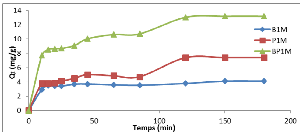
Fig. 4. Effect of contact time on phenacetin adsorption by the activated carbons
