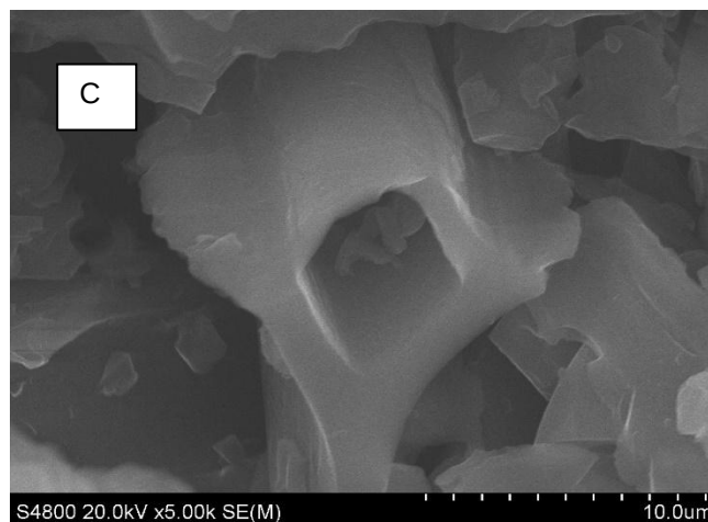
Fig. 1. The SEM photograph of the prepared activated carbons (A: B1M, B: P1M and C: BP1M).
