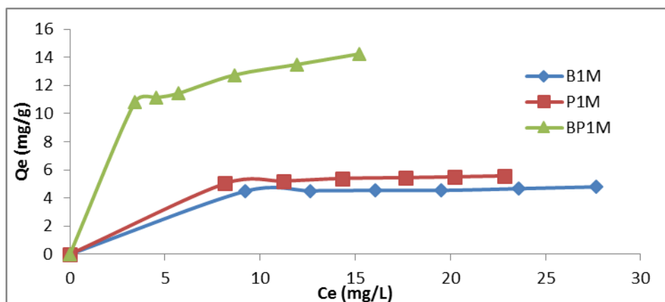
Fig.9. Effect of initial concentration on adsorbed quantities
