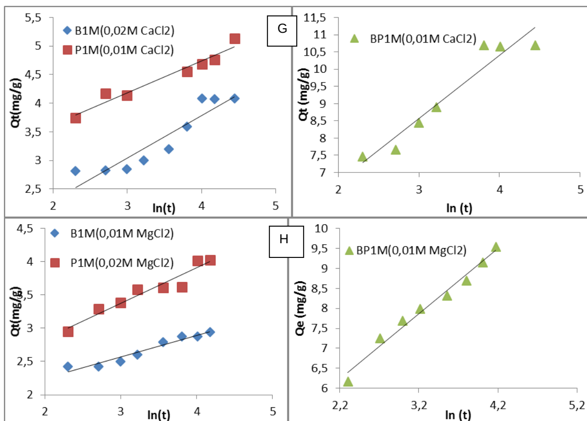
Fig. 7. Linearized pseudo-second order (A: no sel, B: with KCl, C: with CaCl 2 , D: with MgCl 2 ) and Elovich (E: no sel, F: with KCl, G: with CaCl 2 , H: with MgCl 2 ) plots.
