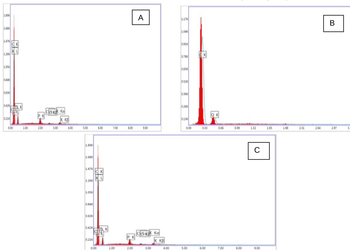
Fig. 2. EDX analysis of the prepared activated carbons (A: B1M, B: P1M and C: BP1M)
