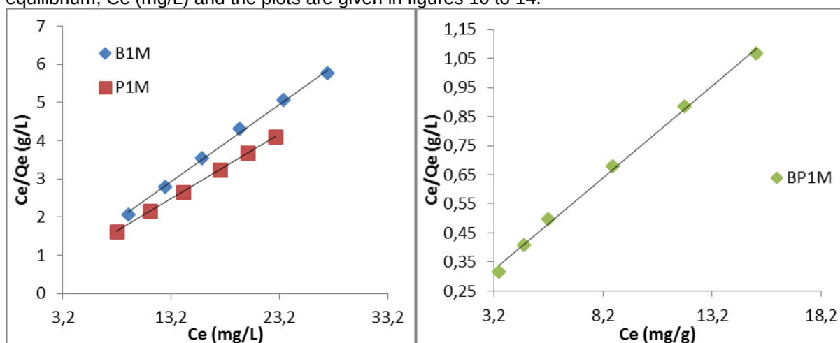
Fig. 10. Linear transformation of Langmuir model
