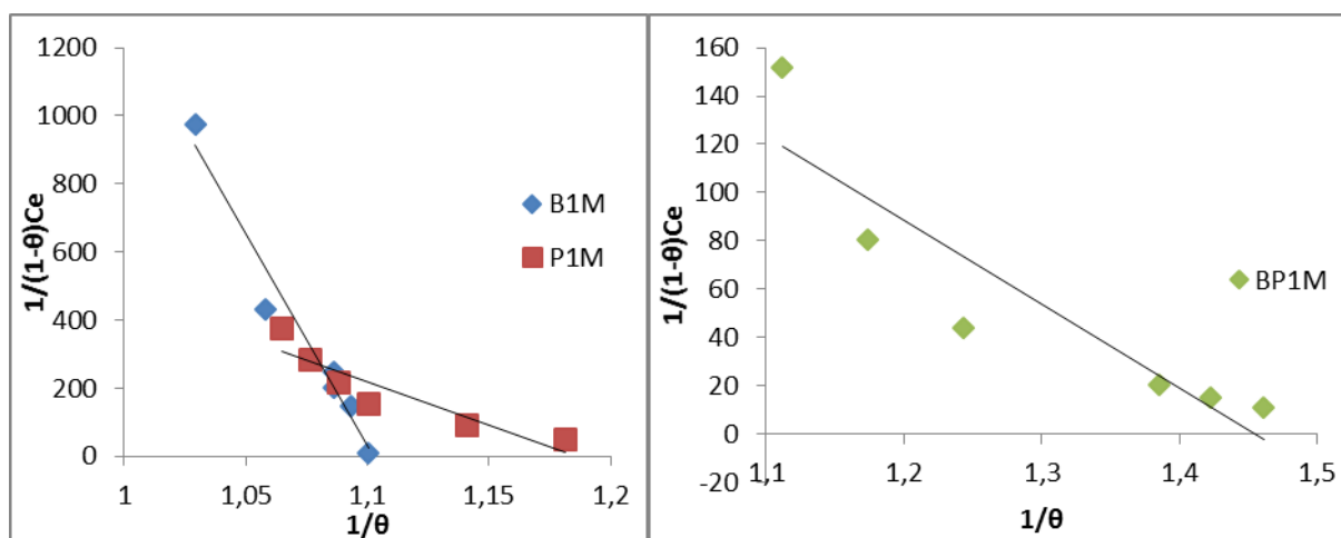
Fig.14. Linear transformation of the Kiselev model
