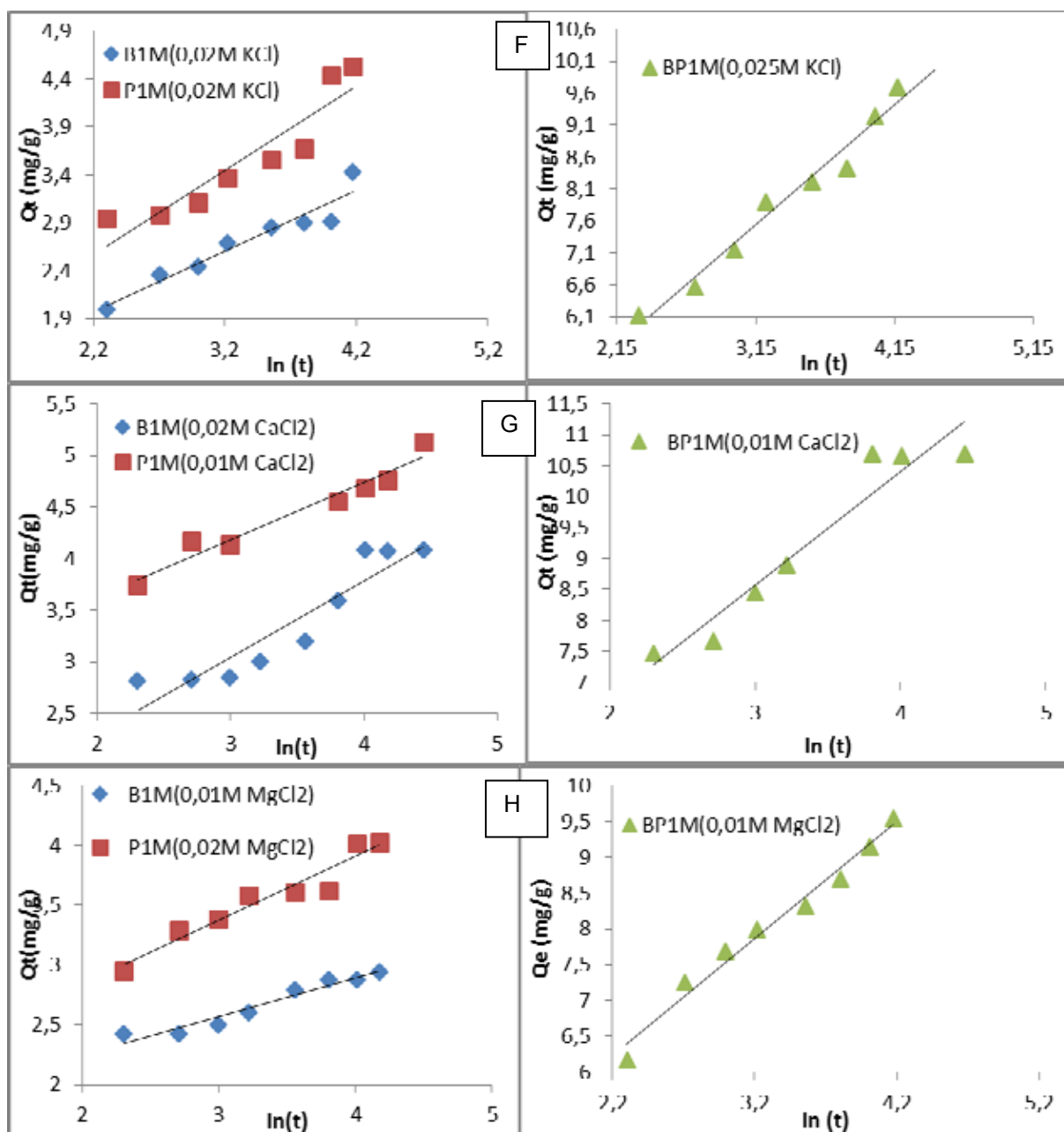
Fig. 7. Linearized pseudo-second order (A: no sel, B: with KCl, C: with CaCl 2 , D: with MgCl 2 ) and Elovich (E: no sel, F: with KCl, G: with CaCl 2 , H: with MgCl 2 ) plots.
