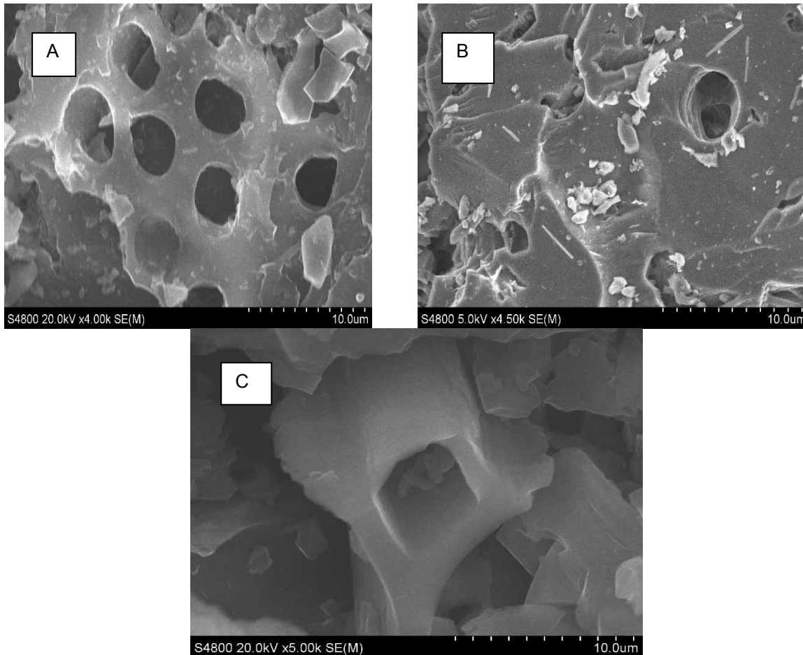
Fig. 1. The SEM photograph of the prepared activated carbons (A: B1M, B: P1M and C: BP1M).
