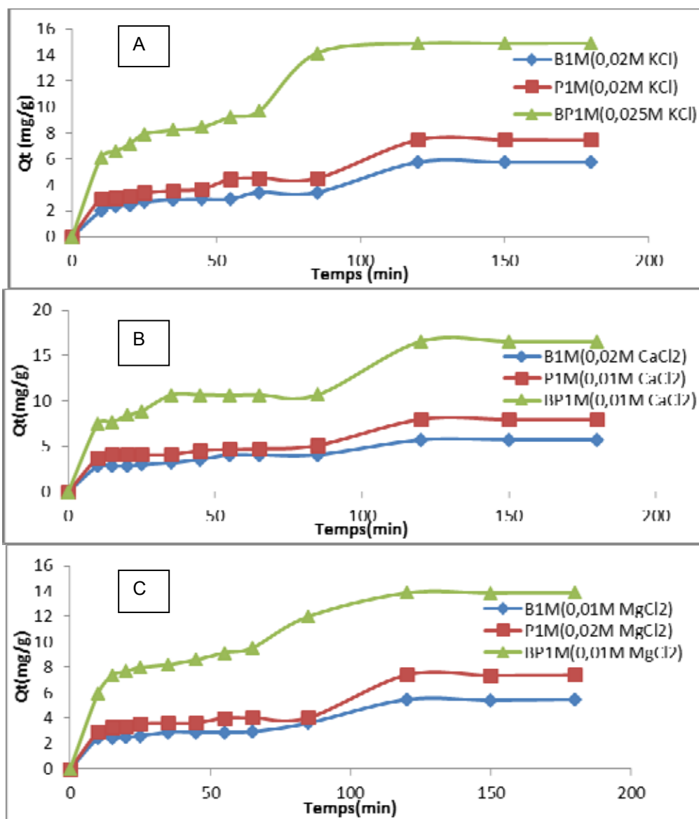
Fig. 6. Effect of salts on the contact time (A: effect of KCl, B: effect of CaCl_2 and C: effect of MgCl_2 )
