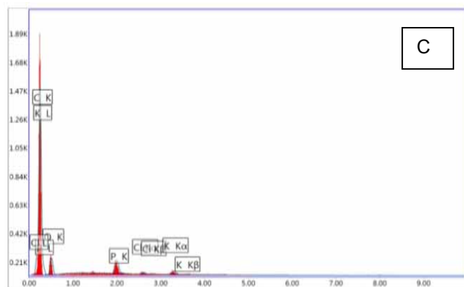
Fig. 2. EDX analysis of the prepared activated carbons (A: B1M, B: P1M and C: BP1M)
