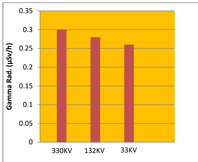
Figure 4: Gamma Rad. from different Units of Mando Sub- station
