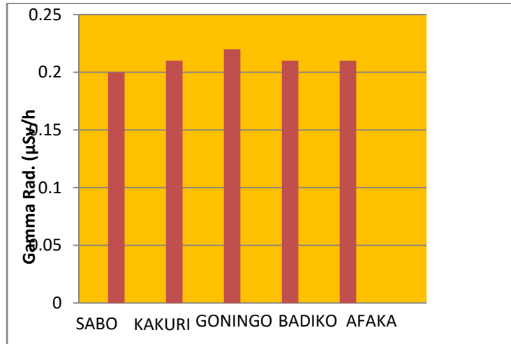
Figure 1: Variation of Gamma Rad. from different locations for 11KV Power line
