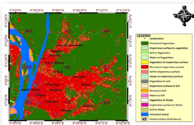
Figure 10: LU/C Transition Map of Onitsha Metropolis between 2016 and 2031.
