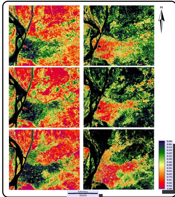
Figure 3: LSMA result of unmixed land use/cover maps of Onitsha: Top LHS, Middle LHS and Bottom LHS – Vegetation endmember fractions of 1986, 2001 & 2016, respectively; Top RHS, Middle RHS and Bottom RHS – Impervious surface endmember fractions of 1986, 2001 & 2016
