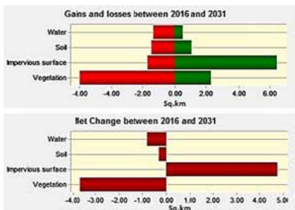
Figure 9: Gains and Losses and Net Change graphs of LU/C classes of Onitsha between 2016 and 2031
