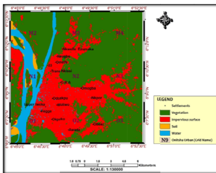
Figure 8: Predicted LU/C map of Onitsha Metropolis (2031)
