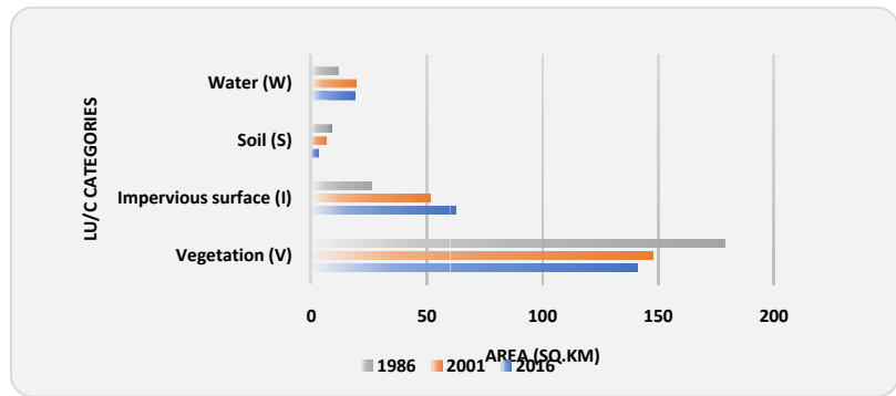
Figure 6: LU/C categories of Onitsha (1986, 2001 & 2016)
