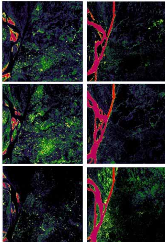
Figure 4: LSMA result of unmixed land use/cover maps of Onitsha: Top LHS, Middle LHS and Bottom LHS – Soil endmember fractions of 1986, 2001 & 2016, respectively; Top RHS, Middle RHS and Bottom RHS – Water endmember fractions of 1986, 2001 & 2016, respectively
