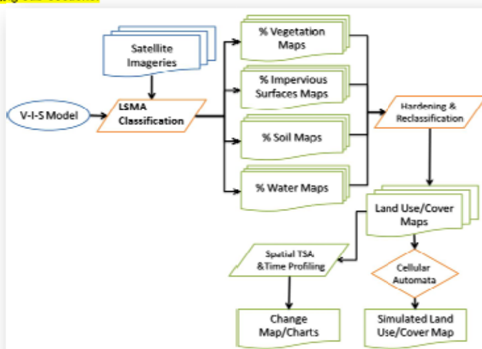
Figure 2: Workflow of the study
