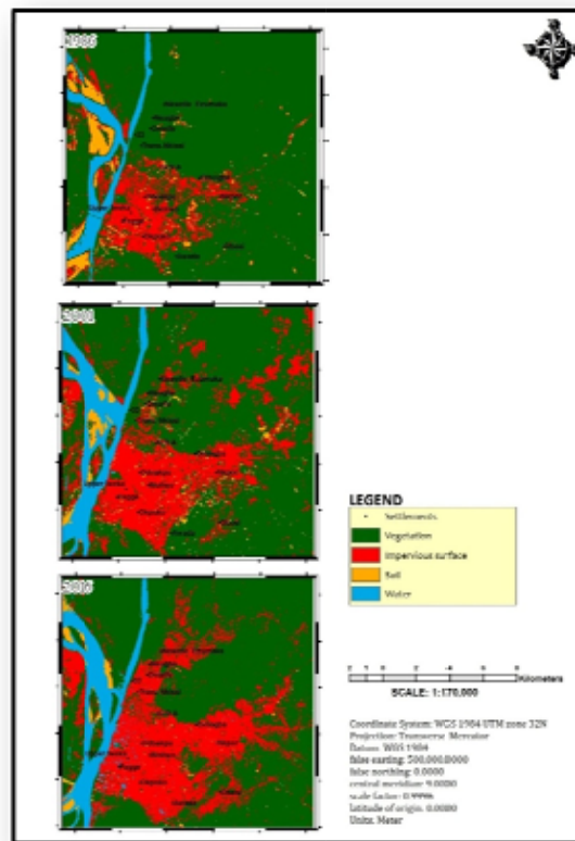
Figure 5: Land use land cover categories of Onitsha (Top: 1986; Middle: 2001; & Bottom: 2016)
