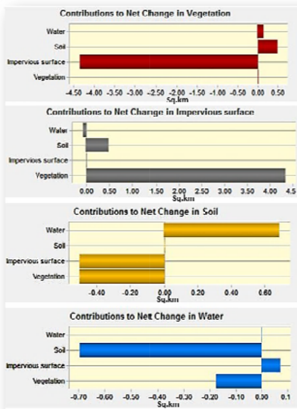
Figure 10: Contribution to Net Change in each LU/C class between 2016 and 2031
