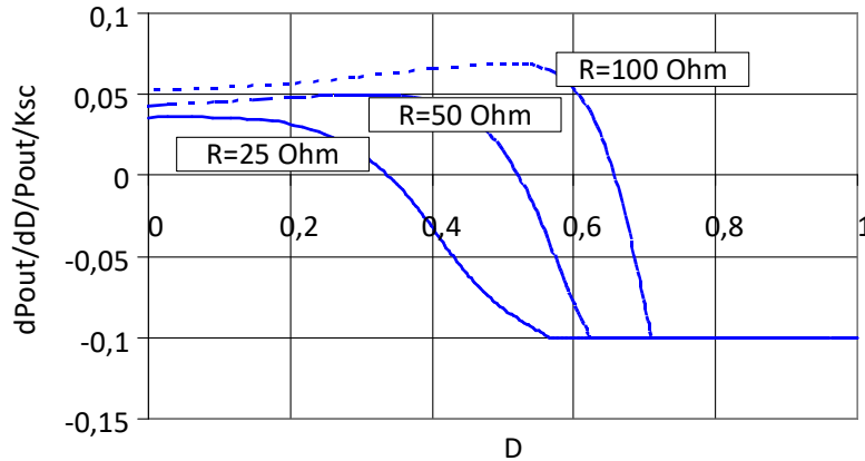
Fig. 10. Modified function for calculation of \Delta D_i for single system.
