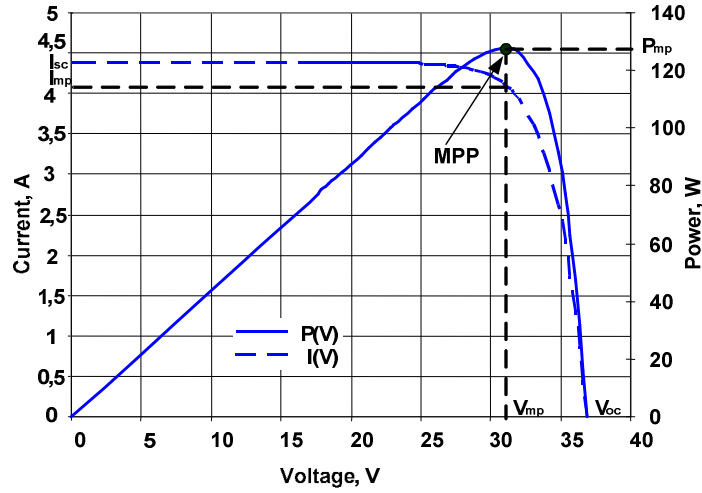
Fig 5. Characteristics curve of a typical PV cell.
