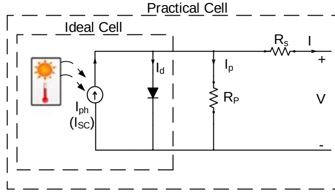
Fig. 2. Equivalent Circuit of Photovoltaic Cell.
