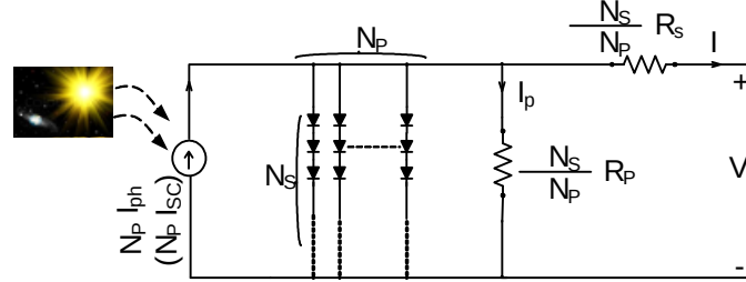
Fig 3. Equivalent circuit model of solar PV array
