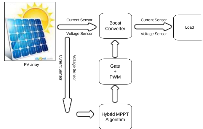
Fig 1. General block diagram of configuration of Solar Power System
