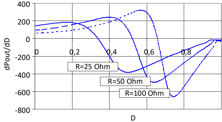
Fig. 9. Dependence dP_{out}/dD from duty cycle D for single system.
