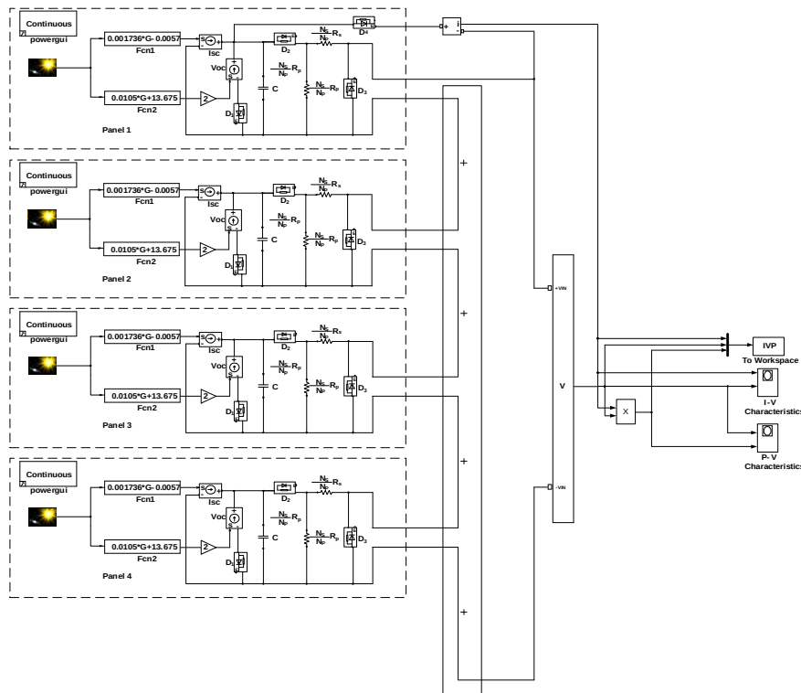
Fig 4. Simulation diagram for of PV array built in SimPowerSystems.
