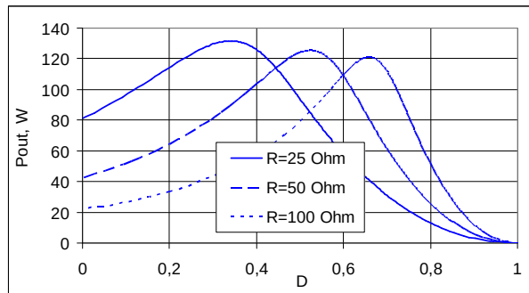
Fig. 8. Dependence P_{out} from duty cycle D for single system.
