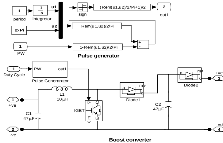
Fig. 7. Simulink-model of Boost DC-DC converter.
