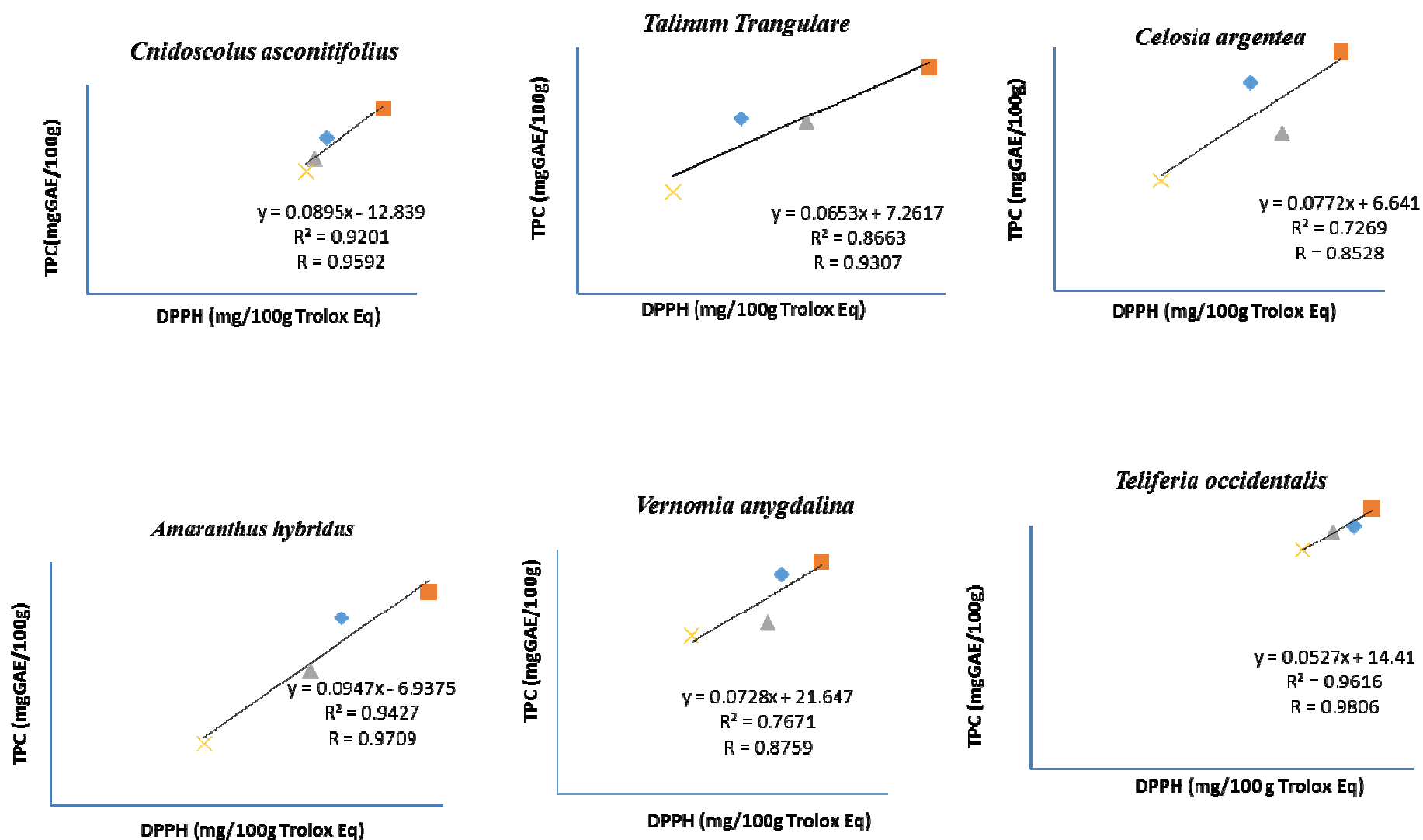
Figure 1; Correlation graph between total phenolic content and antioxidant activities of blanched and raw green leafy vegetables
