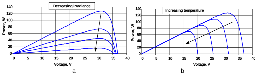
Fig. 1 Impact of factors on power-voltage characteristics of a PV array: a - irradiance; b - temperature
