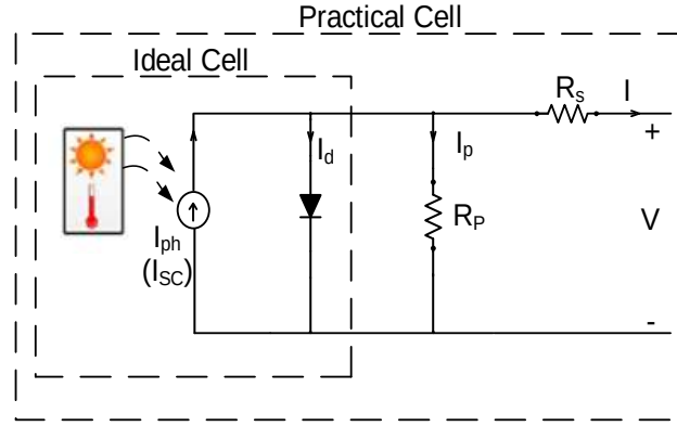
Fig. 2. Equivalent Circuit of Photovoltaic Cell.
