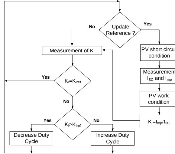
Fig. 5. Flow chart of the K_I
