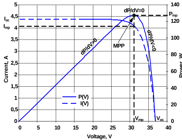
Fig. 5. Perturb and Observe (P & O) Method
