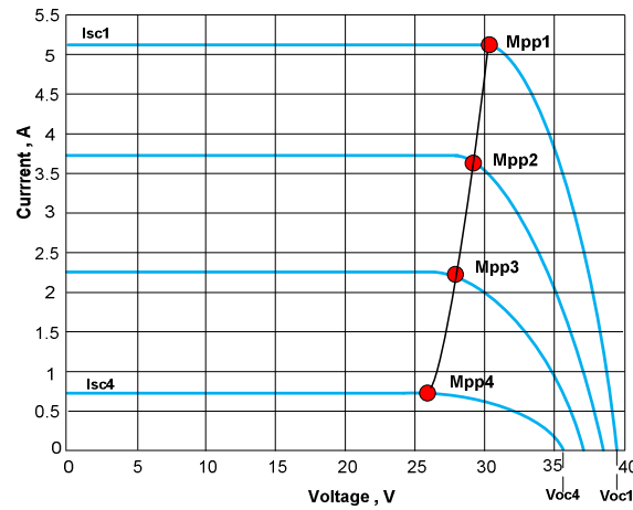
Fig. 3 The I-V characteristics of solar cells under varying sunlight
