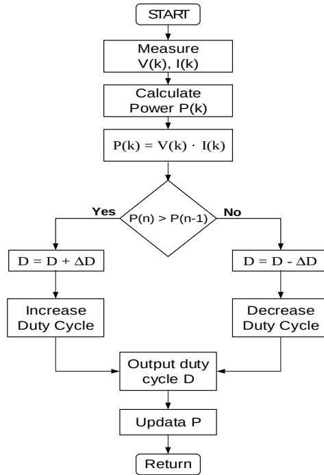
Fig. 10. Flowchart of the hill climbing method
