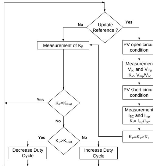
Fig. 6. Flow chart of the K_P
