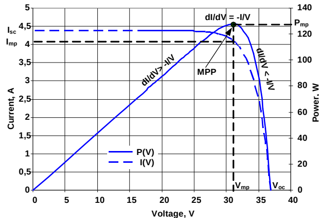
Fig. 7. Incremental Conductance (IncCond) method
