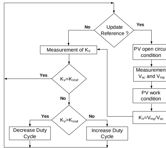
Fig. 4. Flow chart of the K_V
