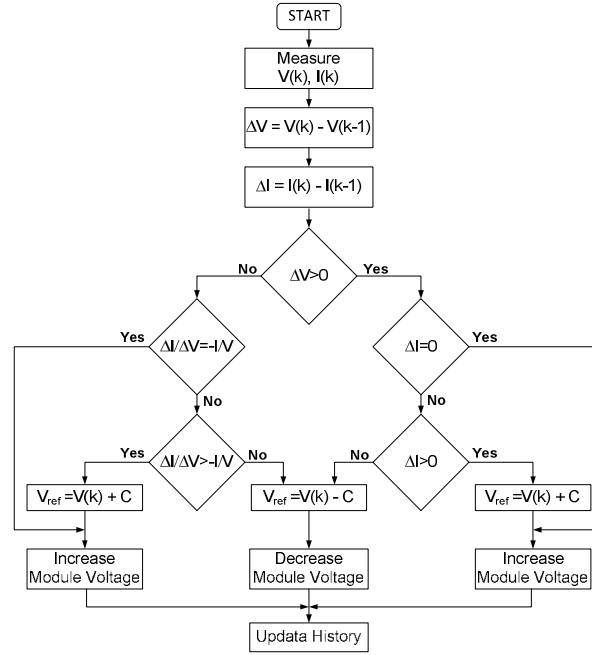
Fig. 8. Flowchart of incremental conductance (IncCond) method
