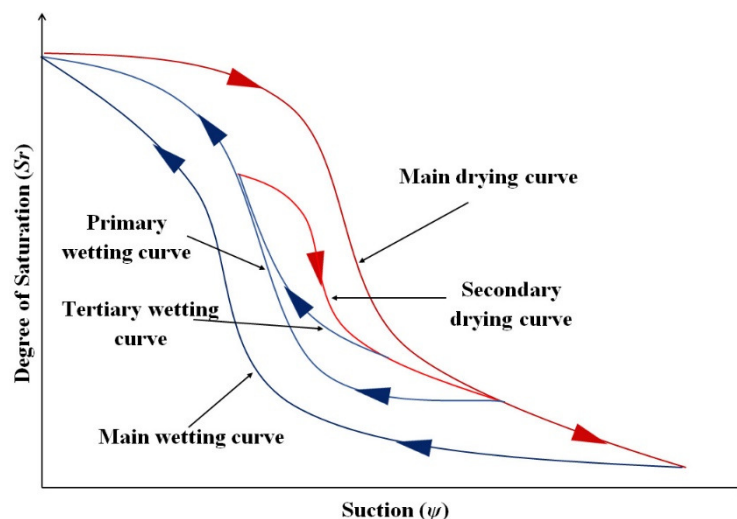
Fig. 2. Primary, secondary and tertiary wetting and drying paths of unsaturated soil [25].
