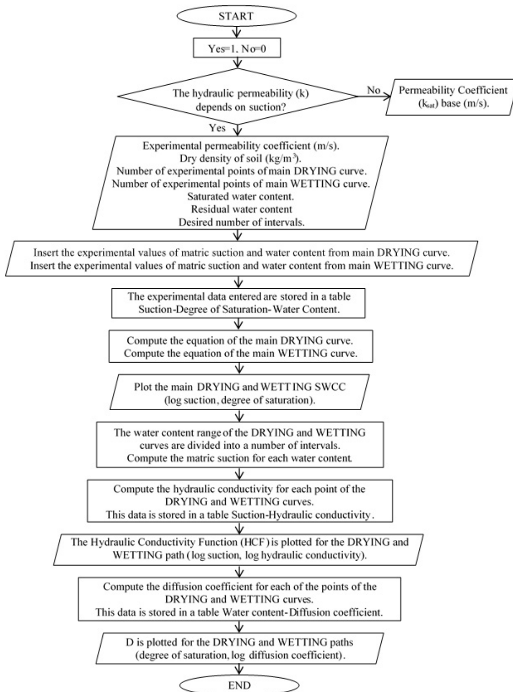
347 348 349 350 Fig. 3. Flow chart for the estimation of the hydraulic parameters of unsaturated soils. 351
