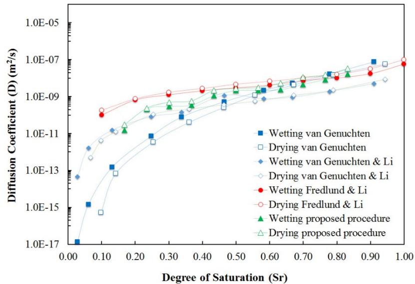
479 480 481 482 Fig. 9. Comparison of diffusion coefficient obtained from different methods using the 483 SWRC reported by Lu and Likos [16]. 484 485
