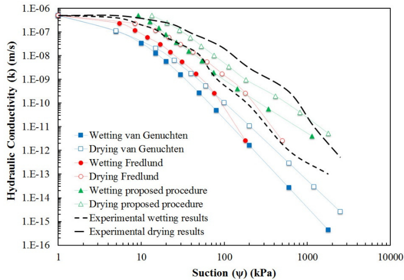
448 449 450 451 Fig. 8. Comparison of hydraulic conductivity obtained from different methods using 452 the SWRC reported by Lu and Likos [16].
