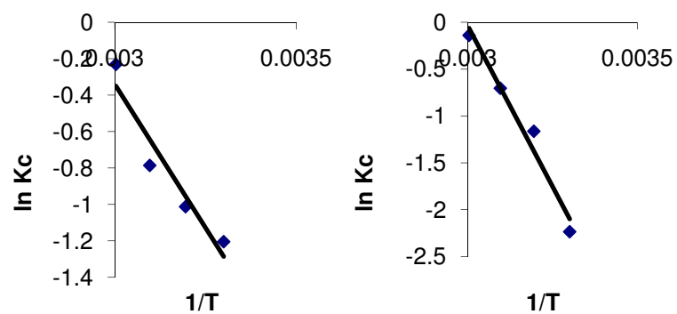
Figure 9: Thermodynamic plot for the adsorption of 4NP onto PSD in (a) binary(4NP+5C-Ph) and (b) ternary (4NP + 5-Ph + 5-C-Ph) system.
