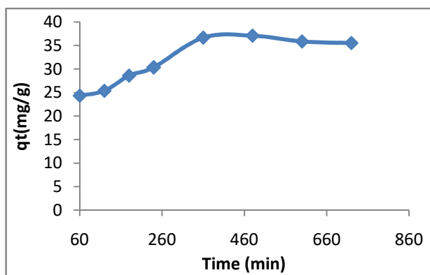
Figure 6: Effect of contact time on the adsorption of 4NP on PSD
