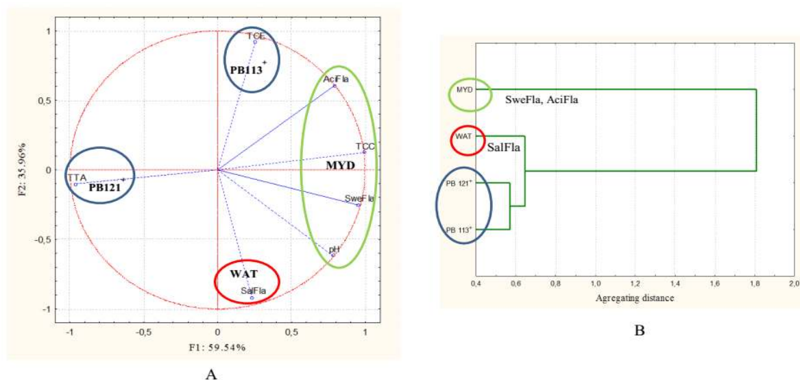
Fig 3. Correlations between the studied coconut sap samples and their sensory and related physicochemical parameters in the F1-F2 factorial draw of the PCA (A) and clustering dendrogramme of the coconut sap samples (B).
