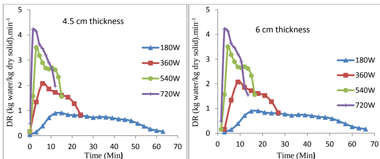
Fig 2 Relationship between the drying rate (kg water/kg dry solid).min -1 and drying time (min) at different bed thickness (1.5, 3, 4.5, 6 cm) and microwave power (180, 360, 540, 720 W)
