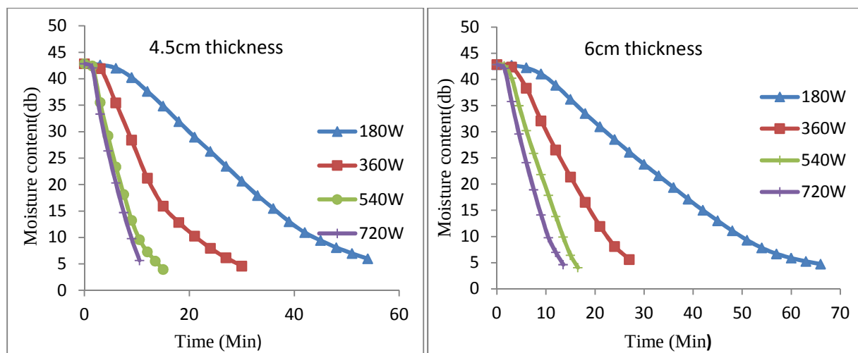
Fig 1 Relationship between the moisture content (kg of water/ kg of dry matter) and drying time (Min) at different bed thickness (1.5, 3, 4.5 and 6 cm) and microwave power (180, 360, 540 and 720 W)
