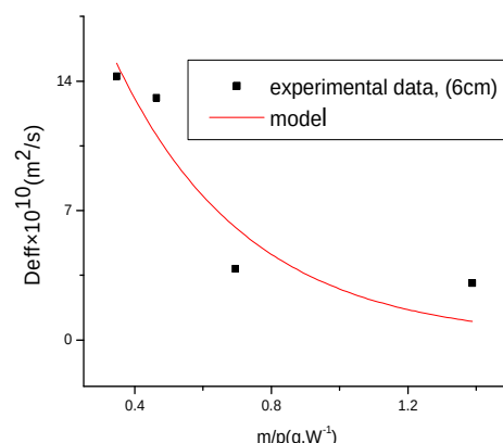
Fig.4 Relationship between effective moisture diffusivity and sample amount/power
