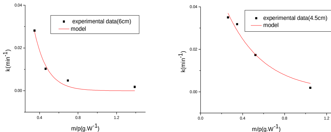
Fig.3 Relationship between the values of drying rate constant and sample amount/power.
