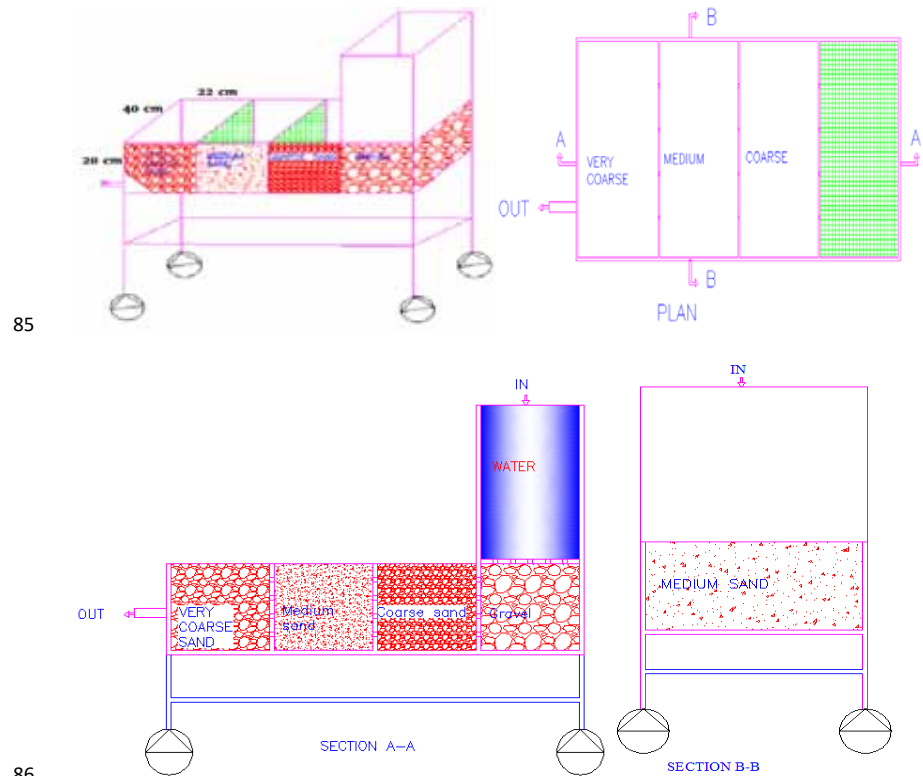
86 87 Figure 1: Horizontal slow sand filtration tool sections/views
