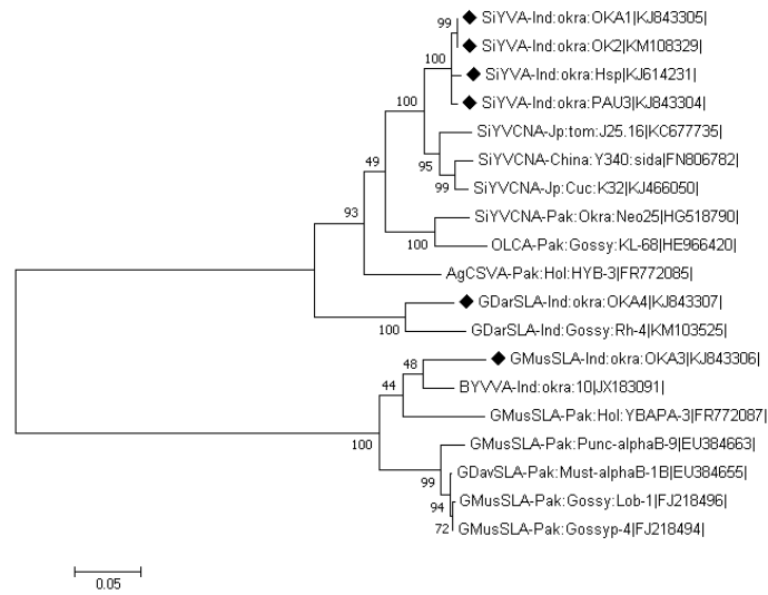
Figure 4: Maximum likelihood tree was depicted from cloned alphasatellite sequences produced in this study (labeled with black diamond) and selected alphasatellite sequences obtained from the database under TN93 model (BIC = 14638.95; INL = -7124.56; AIC = 1427.27; freqA = 0.296; freqT = 0.284; freqC = 0.195; freqG = 0.223; R = 1.235). The tree is unrooted and the number on nodes represent percentage bootstrap values (1000 replicates).
