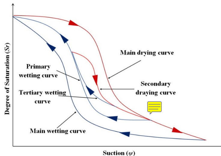
Fig.2. Primary, secondary and tertiary wetting and drying paths of unsaturated soil [22].
