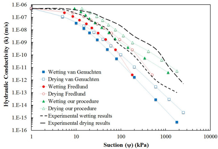
Fig.8. Comparison of hydraulic conductivity obtained from different methods using the SWRC reported by Lu and Likos[16].
