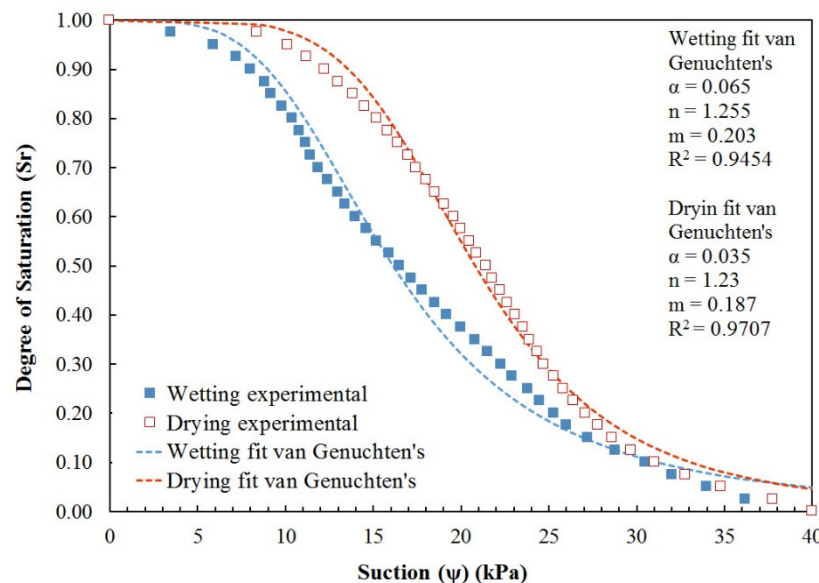
Fig.4. Experimental SWRCs and van Genuchten's fit for a sand reported by Gonzalez and Adams (1980) [7].
