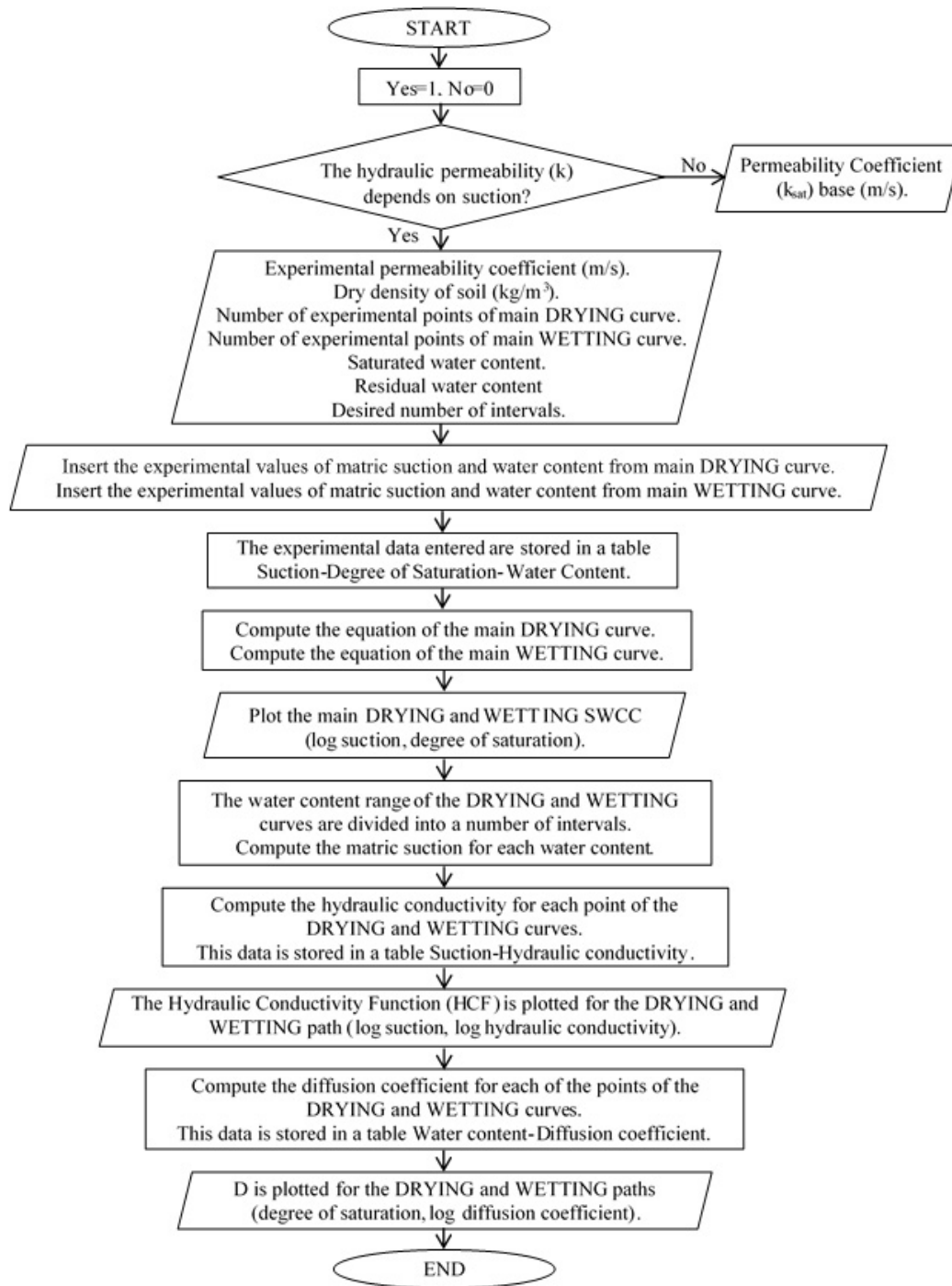
Fig.3. Flow chart for the estimation of the hydraulic parameters of unsaturated soils.
