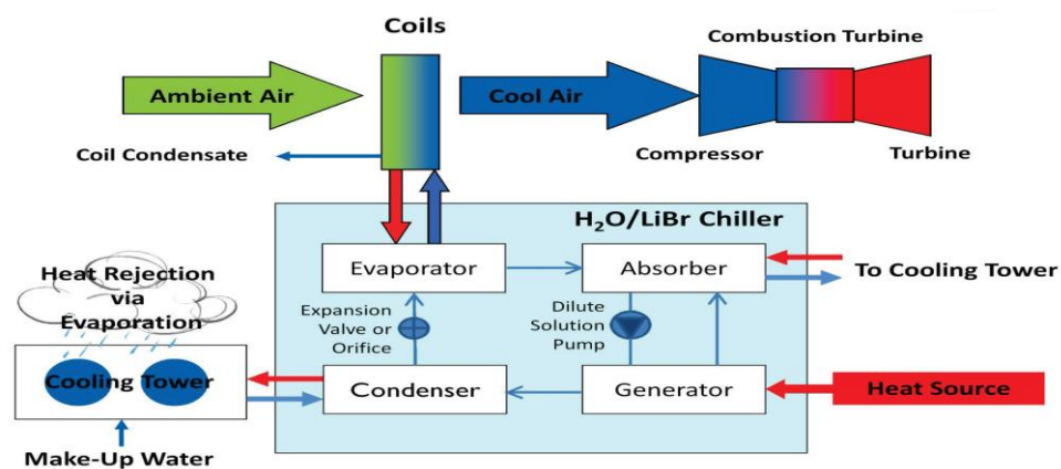
Fig. 1: Typical Turbine Inlet Chilling Process [10]
