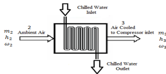
Fig. 4: Typical design of the absorption chiller cooling system.
