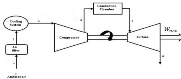
Fig. 3: Schematic diagram of the GT cycle with an inlet air cooler [13]
