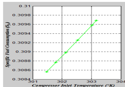
Fig. 12: After Cooling
