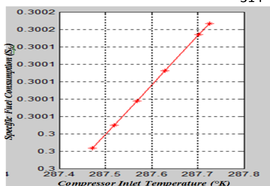
Fig. 11: Before Cooling
