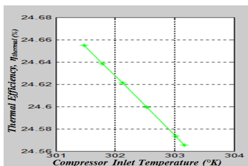
Fig. 7: Before Chilling.
