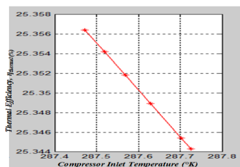
Fig. 8: After Chilling
