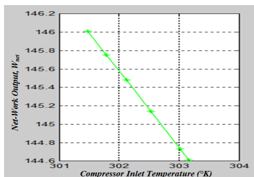
Fig. 9: Before Cooling
