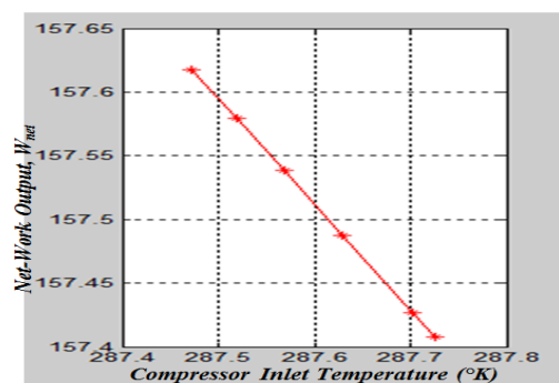
Fig. 10: After Cooling
