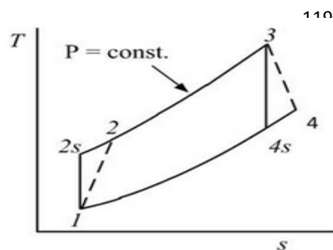
Fig. 3b: T-S Diagram of the GT Cycle [14]
