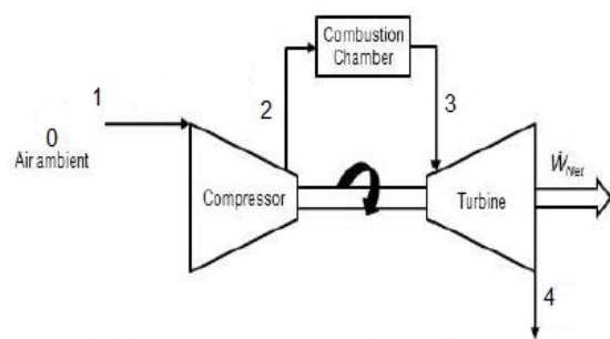
128 Fig. 3a: Simple GT Cycle [13]
