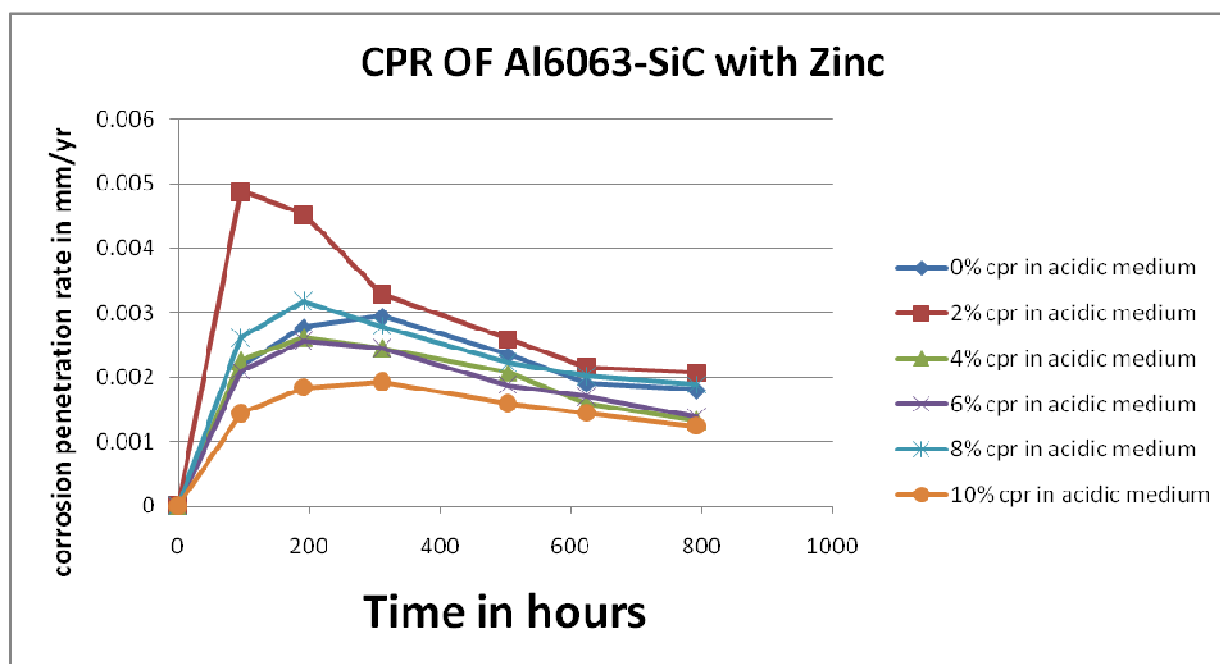
Fig.10: Corrosion Penetration Rate of Al6063-SiC composite with Zinc in an acidic medium
