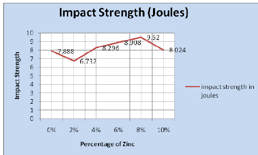
Fig.2: Relationship between the percentage of Zinc in Al6063-SiC-Zn and the Impact Strength of the composite.
