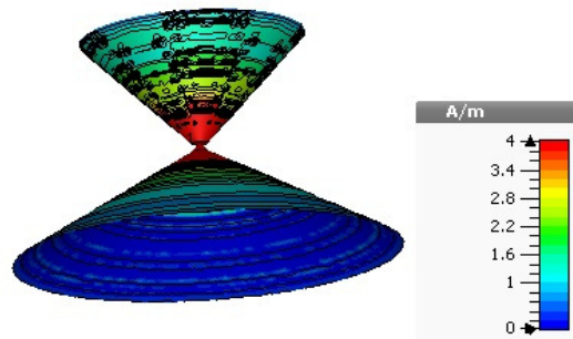
Fig. 3: Biconical Antenna without Edge Termination 25GHz
