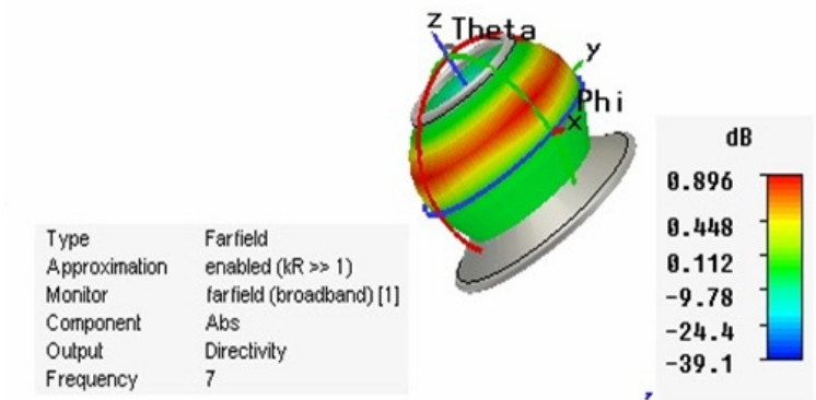
Fig.: 5 Radiation Pattern 3D at 7GHz
