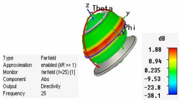
Fig. 6: Radiation Pattern 3D at 25GHz
