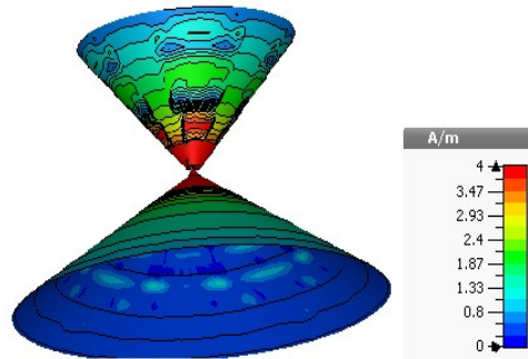
Fig. 1: Biconical Antenna without Edge Termination 6GHz
