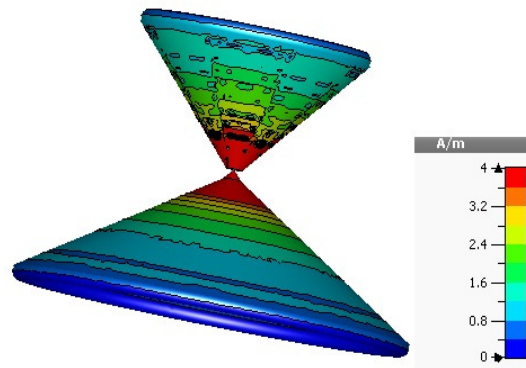
Fig. 4: Biconical Antenna with Edge Termination at 25GHz
