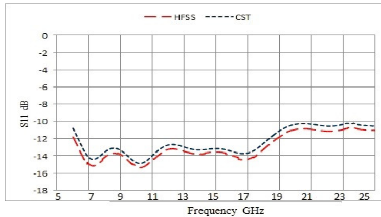
Fig. 10: Frequency Vs. S- parameter with termination
