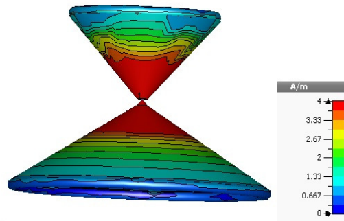
Fig. 2: Biconical Antenna with Edge Termination at 6GHz
