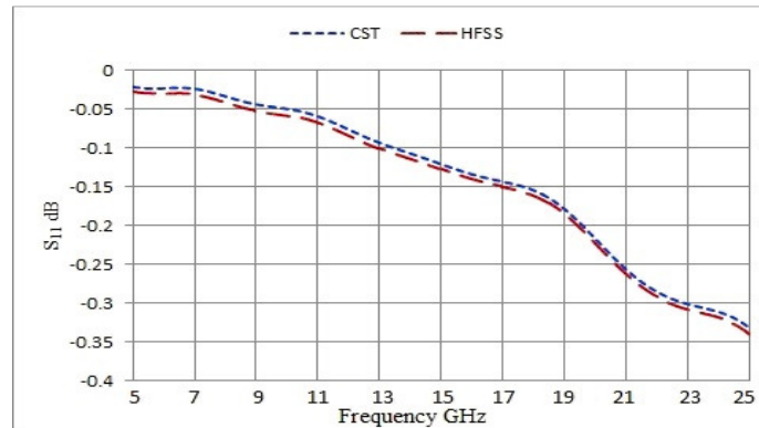
Fig. 9: Frequency Vs .S- parameter without termination
