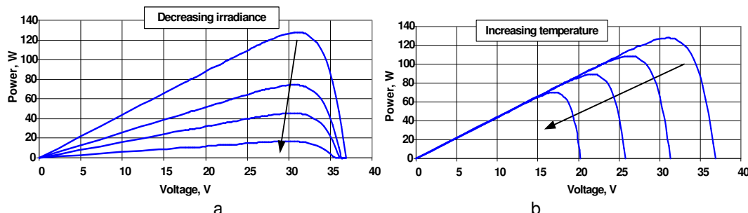
Fig. 2. Impact of factors on power-voltage characteristics of a PV array: a - irradiation; b - temperature
