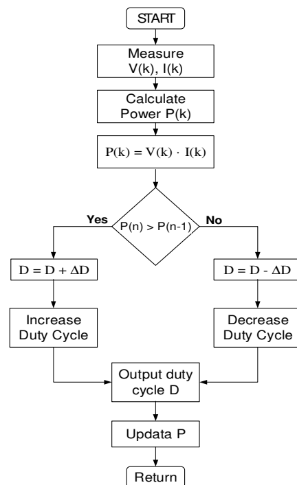
Fig. 10. Flowchart of the hill climbing method
