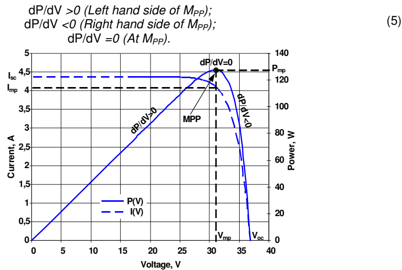
Fig. 5. Perturb and Observe (P & O) Method
