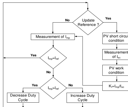
Fig. 4. Flow chart of the SCCF
