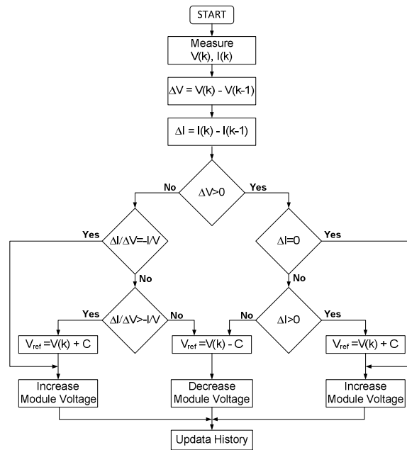
Fig. 8. Flowchart of incremental conductance (IncCond) method
