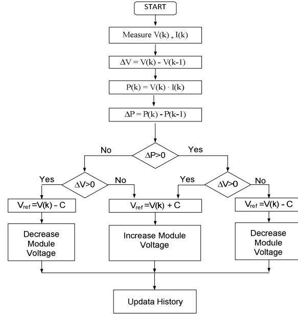
Fig. 6. Flowchart of Perturb and Observe (P & O)
