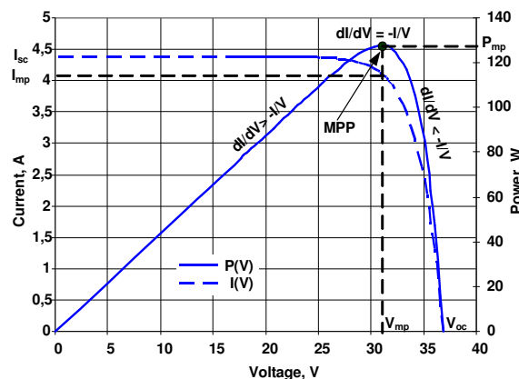
Fig. 7. Incremental Conductance (IncCond) method
