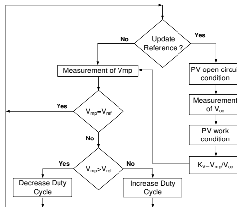
Fig. 3. Flow chart of the OCVF
