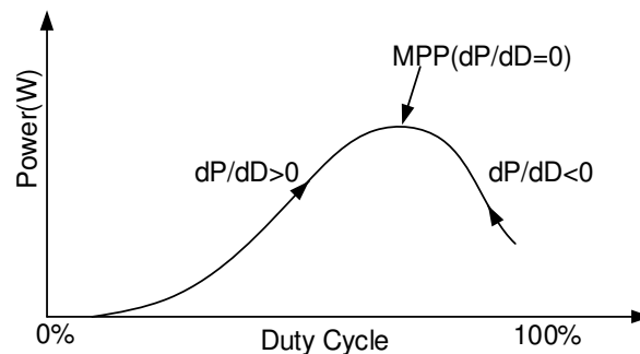
Fig. 9. P-D curve diagram of the hill climbing method
