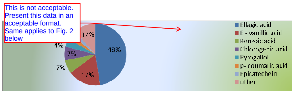
Fig. 1. Percentage of some main phenolic compounds derived from ethanolic hawthorn leaves extract
