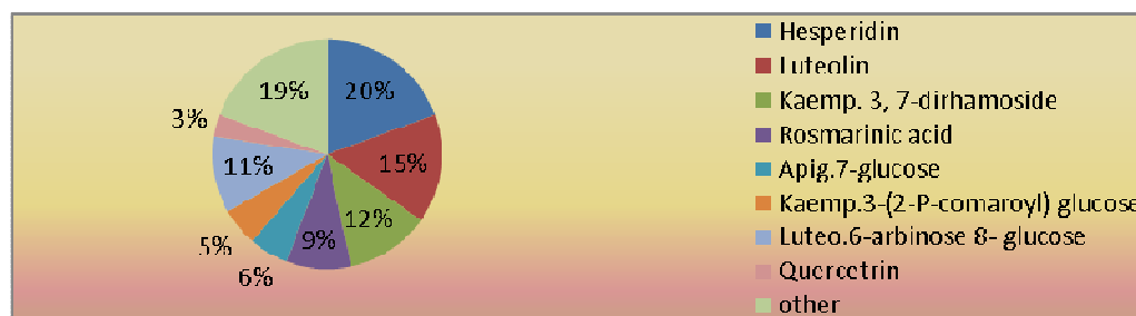
Fig. 2. Percentage of some main flavonoid compounds derived from ethanolic hawthorn leaves extract
