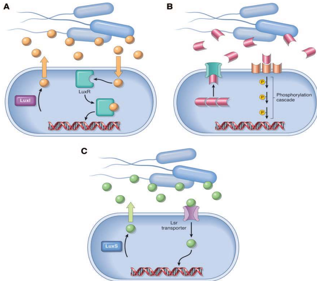
Figure 1: Schematic representation of quorum sensing signaling pathways. The bacteria synthesize and released the AIs (regardless of their chemical nature) which will diffuse to the surrounding environment until they reach a certain threshold concentration; then they will diffuse back to the cell, bind to a specific receptor and activate the transcription of target genes. A; LuxI/R in Gram negative bacteria. B; AIP in Gram positive bacteria. In this model, the AIs will not diffuse back into the cells; instead, they will bind to a surface receptor which will induce a signal transduction cascade that will ultimately result in altered gene expression. C; LuxS/Lsr transporter in Gram negative and Gram positive.
