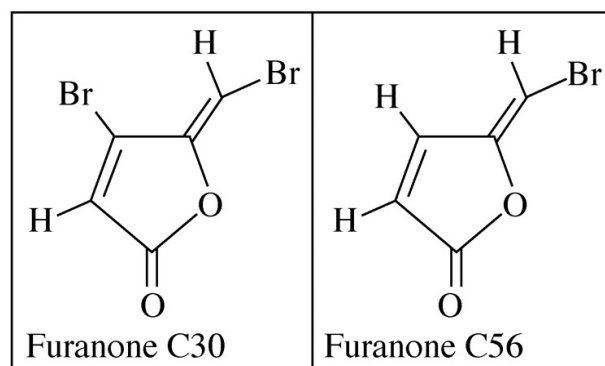
Figure 3: structure of furanones C30 and C56
