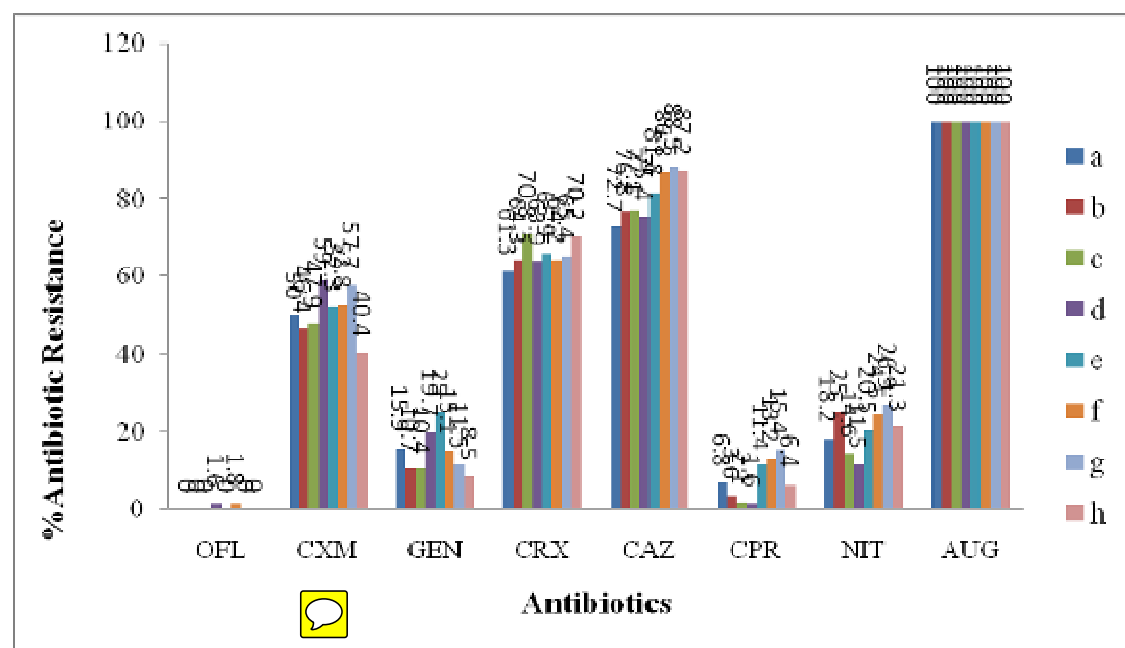
Fig. 2: Antibiotic resistance of Escherichia coli isolated from food samples obtained from food outlets in Ekiti State University and Environ.
