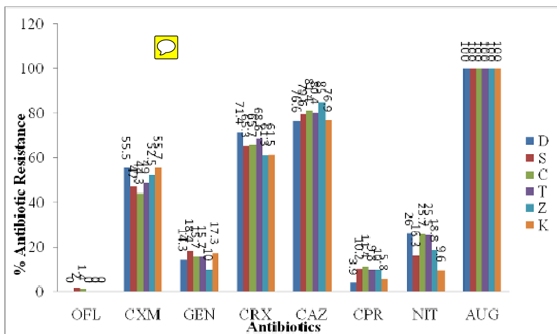
Fig. 1: Antibiotic resistance of the Escherichiacoli isolated from food outlet in Ekiti State University and Environ.
