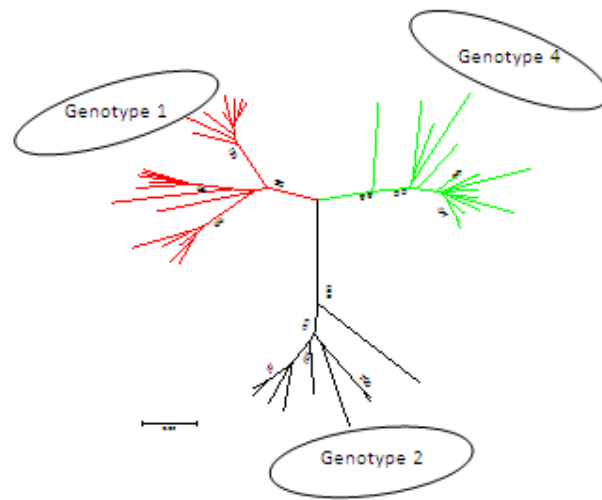
Figure 1a: Neighbour joining (NJ) tree of the C region of HCV isolated from Cameroon In Red; Genotype 1 sequences, in Green : Genotype 4 sequences and in Black: Genotype 2 sequences
