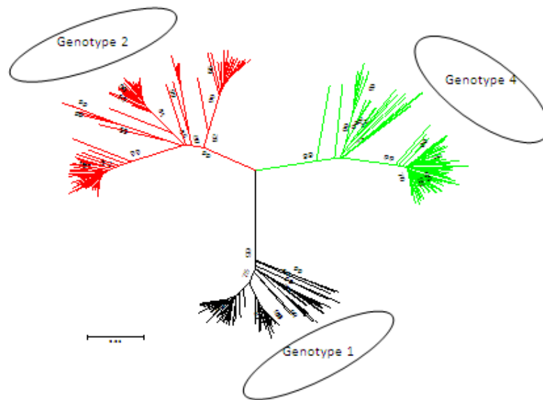
Figure 1c: Neighbour joining (NJ) tree of the NS5B region of HCV. Each colour represents a specific genotype.
