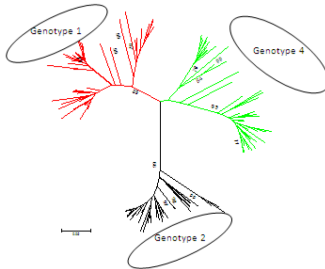
Figure 1b: Neighbour joining (NJ) tree of the E1 region of HCV. Each colour represents a specific genotype. In Red; Genotype 1 sequences, in Green : Genotype 4 sequences and in Black: Genotype 2 sequences
