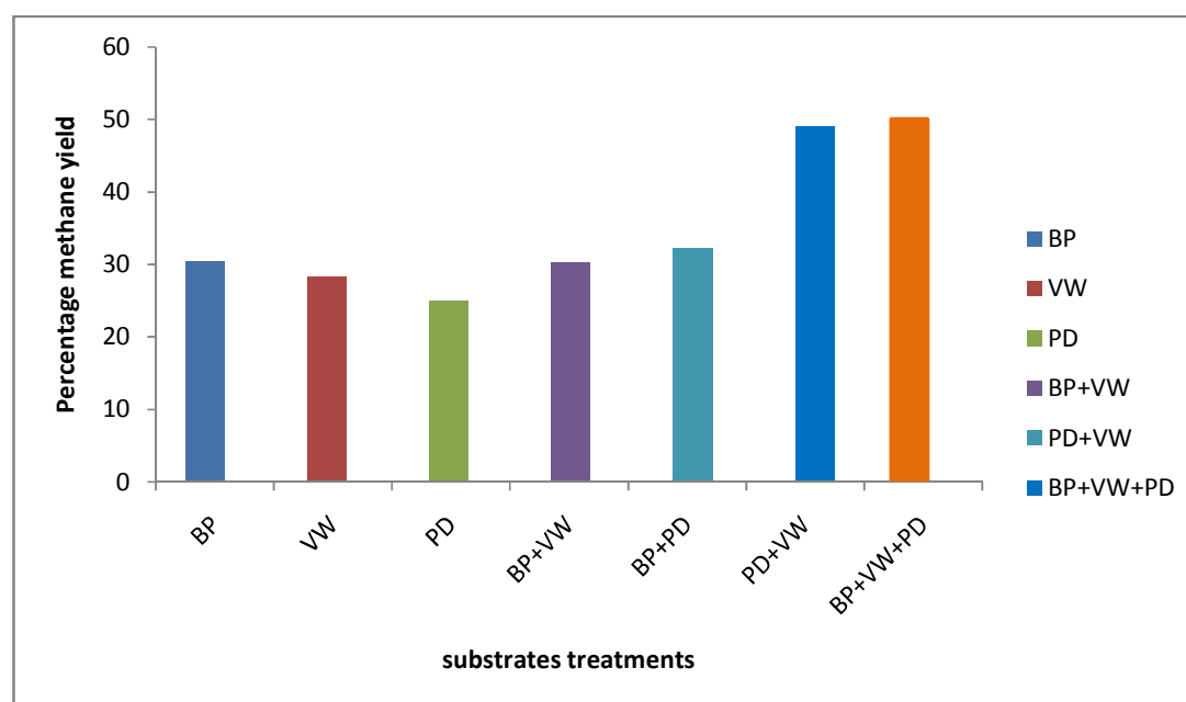
Fig 7: Percentage methane yield during anaerobic digestion of substrates at varying retention time
