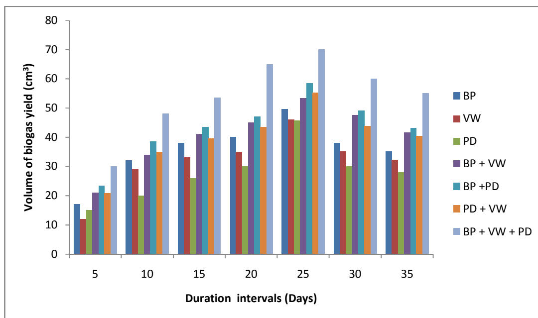
Fig 5: Mean biogas yield during anaerobic digestion of substrates at varying retention time (5-35 days)
