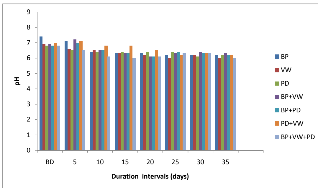
Fig. 2: Mean pH variations of substrates before digestion (BD) and during anaerobic digestion
