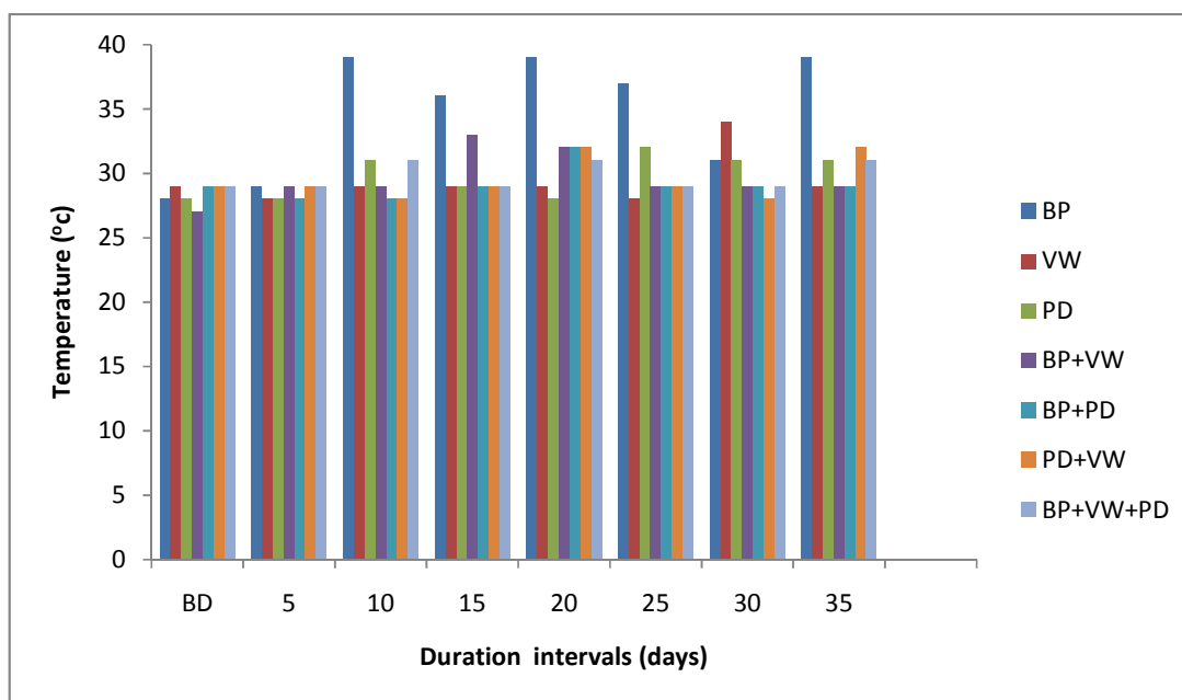
Fig1: Mean temperature variations of substrates before digestion (BD) and during anaerobic digestion
