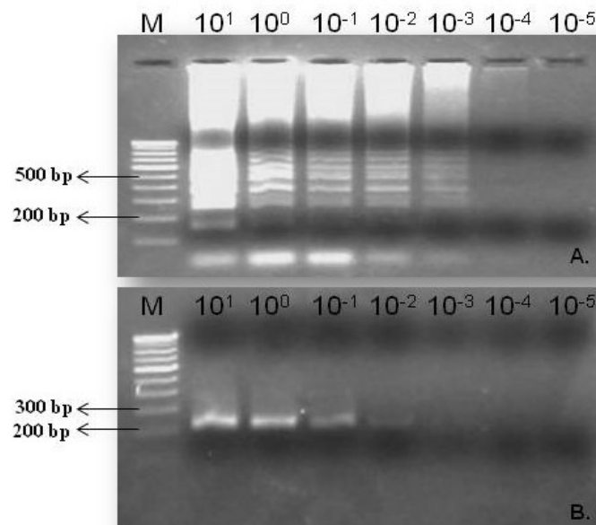
Fig. 5. Sensitivity of RT-LAMP in comparison to conventional RT-PCR. Influenza A virus strain (A/New Caledonia/20/99 (H1N1-like), with known titre of 3 \times 10^3 PFU/ \mu l, was diluted ten-fold serially and detected with RT-LAMP (gel A) and conventional RT-PCR (gel B).
