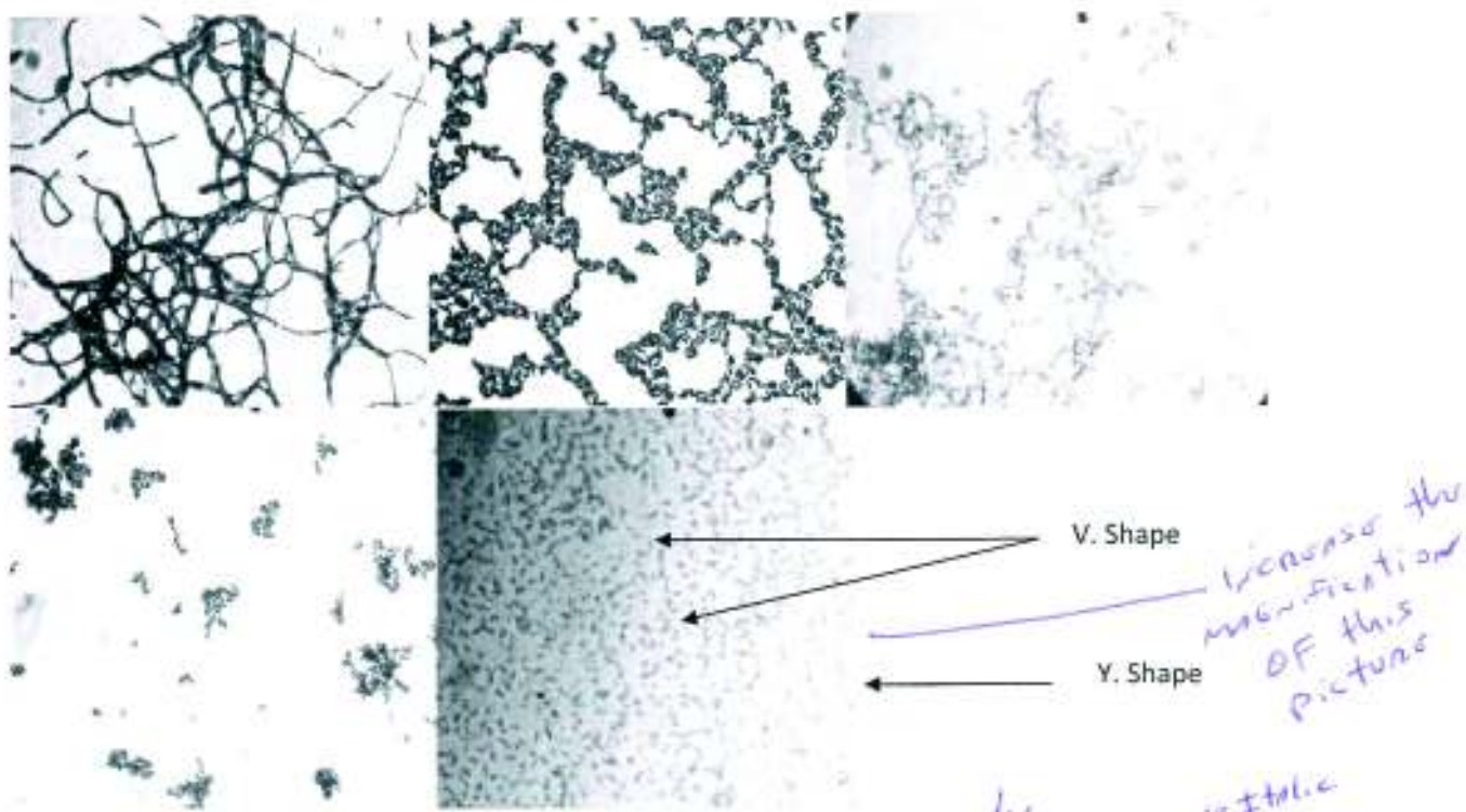
Fig. 2: Cell Morphology of isolates: a-d). Representative of different species of Lactobacillus spp. e). "V" and "Y" shape Bifidobacteria sp. at X1000 magnification.
