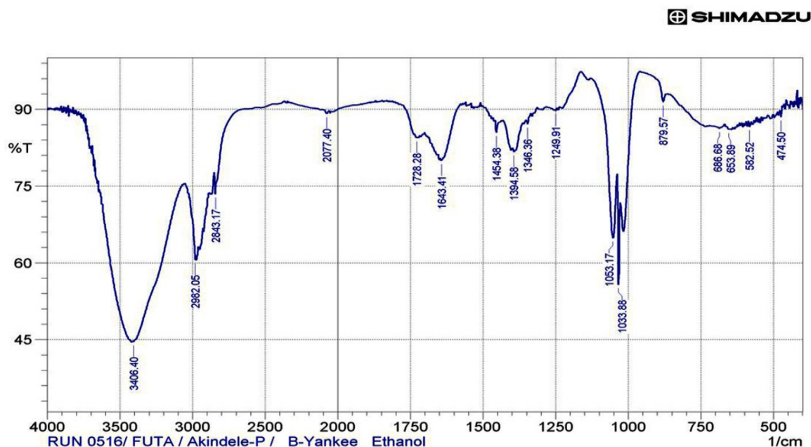
295 Figure 3: Infra-red spectrum of Ethanol fraction showing different peaks
