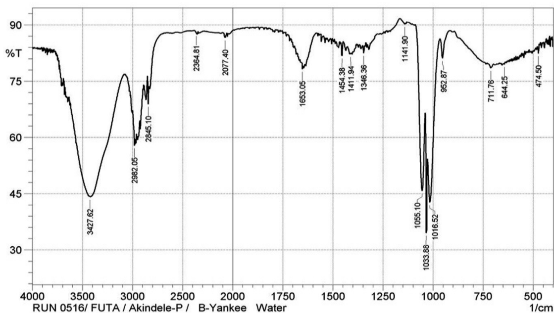
Figure 4: Infra-red spectrum of Cold water extract fraction showing different peaks
