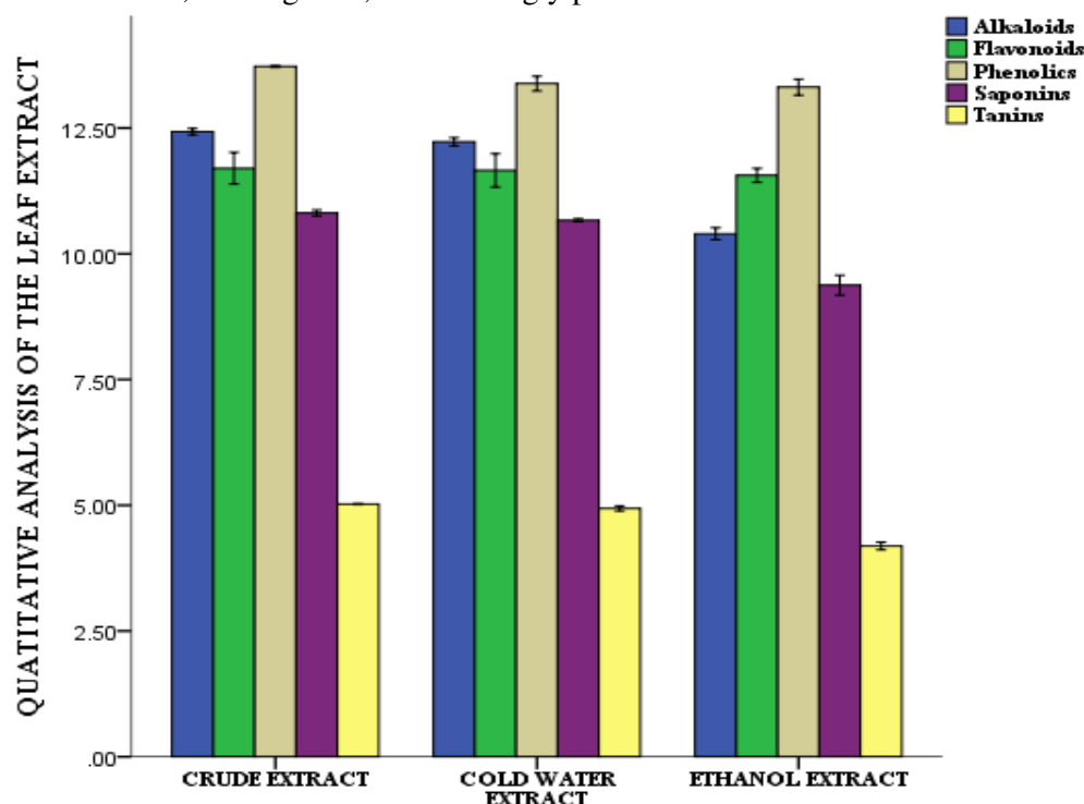
Figure 2: Quantitative phytochemical constituent of Calotropis procera leaf extract Thin Layer Chromatography
