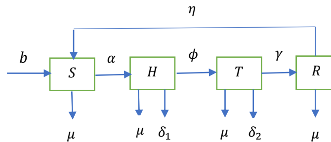
Figure 1: Schematic diagram of the four drinking classes in the model.
