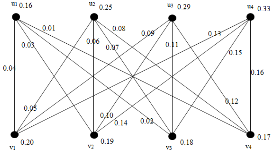
Fuzzy graceful labelling graph K_{4,4}
