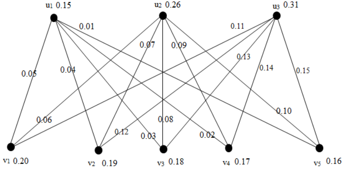
Fuzzy graceful labelling graph K_{3,5}
