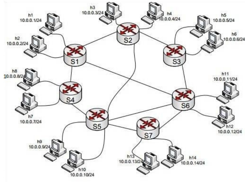
Fig-2: Network Topology
