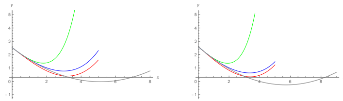
Figure 3: Details of the graphs of the majorizing functions \phi_S(t) (blue), \phi_W(t) (green), \phi_G(t) (red) and \phi_K(t) (gray), for cases of the Orthosie satellite, ( e = 0.243 ), (left) and Themisto satellite, ( e = 0.212 ), (right).
