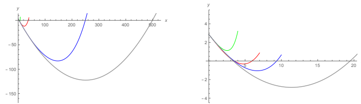
Figure 4: Details of the graphs of the majorizing functions \phi_S(t) (blue), \phi_W(t) (green), \phi_G(t) (red) and \phi_K(t) (gray), for cases of the Enceladus satellite, ( e = 0.004 ), (left) and Europa satellite, ( e = 0.096 ), (right).
