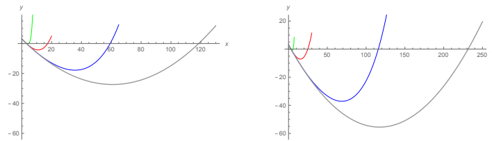
Figure 2: Details of the graphs of the majorizing functions \phi_S(t) (blue), \phi_W(t) (green), \phi_G(t) (red) and \phi_K(t) (gray), for cases of the planet Earth, ( e = 0.0167 ), (left) and planet Neptune, ( e = 0.0086 ), (right).
