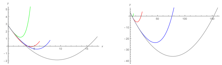
Figure 1: Details of the graphs of the majorizing functions \phi_S(t) (blue), \phi_W(t) (green), \phi_G(t) (red) and \phi_K(t) (gray), for cases of the 1994 JR_1 satellite, ( e = 0.12 ), (left) and 2000 PV_{29} , satellite, ( e = 0.013 ), (right).
